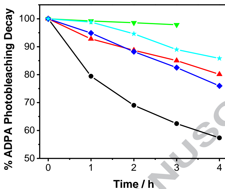
Figure S10. Percentage decay of ADPA photobleaching at \lambda = 378 nm following irradiation (400 – 500 nm) of: PR-SH (black line) PR-AuNP (red line), PR-AuNP-PEG (biphasic) (green line), PR-AuNP-PEG (monophasic) (blue line) and PR-AuNP-PEG-Ab (cyan line). The percentage decay of ADPA photobleaching for PR-SH and PR-AuNP was performed in DCM while for PR-AuNP-PEG and PR-AuNP-PEG-Ab the photobleaching was measured in an aqueous solution.
