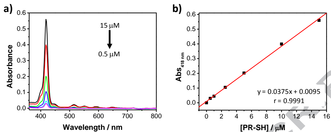
Figure S4. a) UV-Vis absorption spectra of PR-SH at varying concentrations (from 0.5 to 15 \mu\text{M} ) and b) resulting calibration curve plotting the absorbance at \lambda = 418 nm (Soret band) as a function of the concentration of PR-SH .
