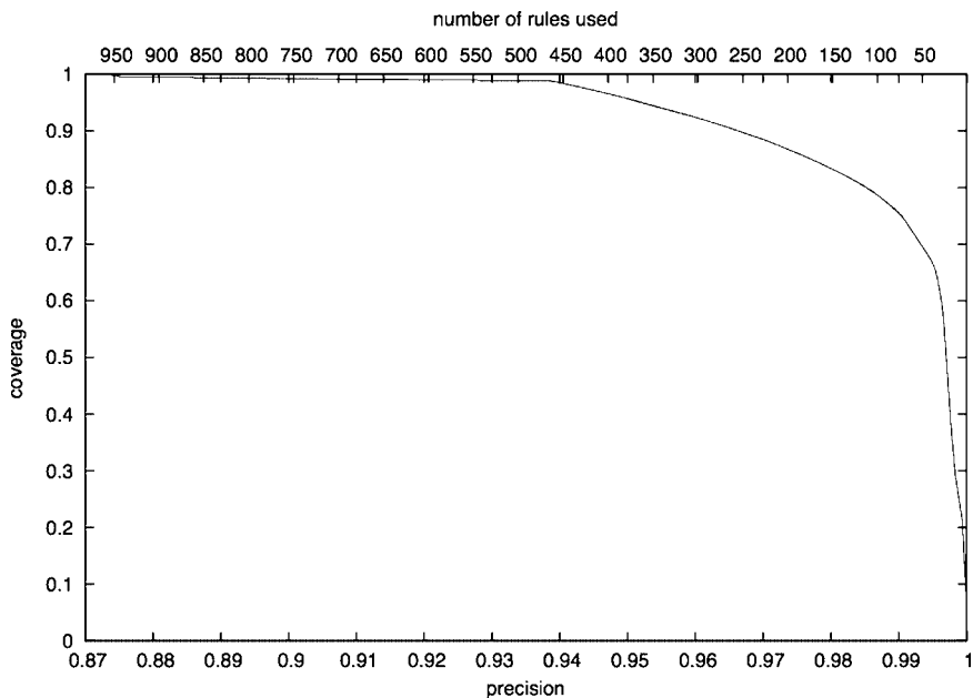
Figure 4 Precision/coverage plot for different rules thresholding of the SEAFR model.
