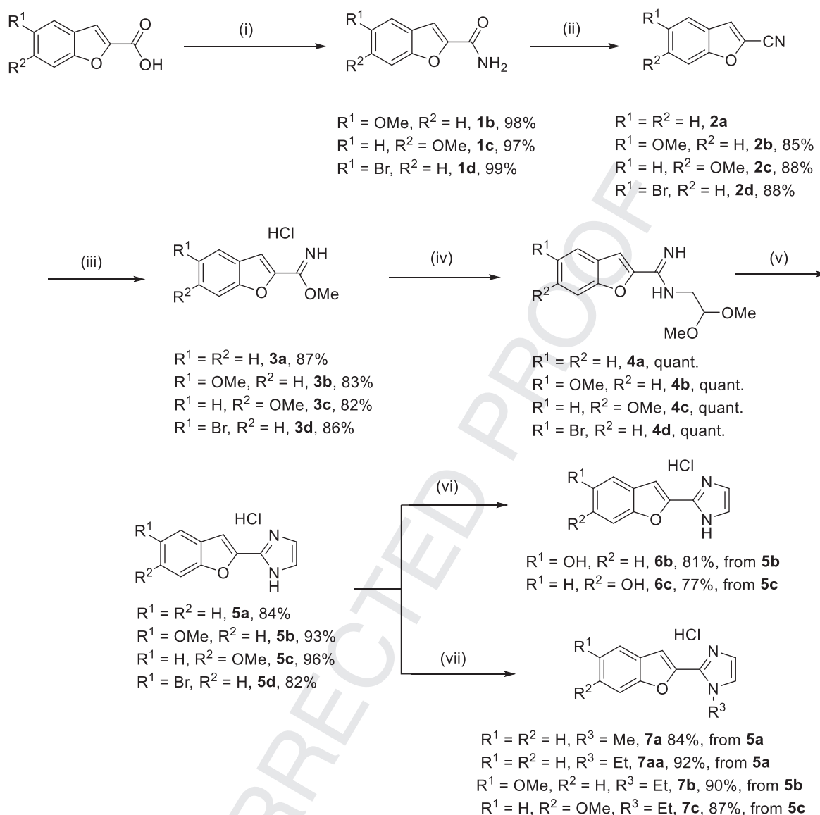
Scheme 1. Reagents and conditions: (i) \text{SOCl}_2 , toluene, 3 h, reflux; 25% aq. \text{NH}_4\text{OH} , rt; (ii) \text{POCl}_3 , dichloroethane, 75 °C, 2 h; (iii) \text{Et}_2\text{O}:\text{HCl} 2 M, 4 °C, 48 h; (iv) 2,2-dimethoxyethylamine, methanol, 60 °C, 16 h; (v) HCl 2 M, 60 °C, 16 h; (vi) HBr 47%, 100 °C, 7 h; (vii) NaH, methyl iodide or ethyl bromide, DMF, 0 °C to rt, 75 min.
