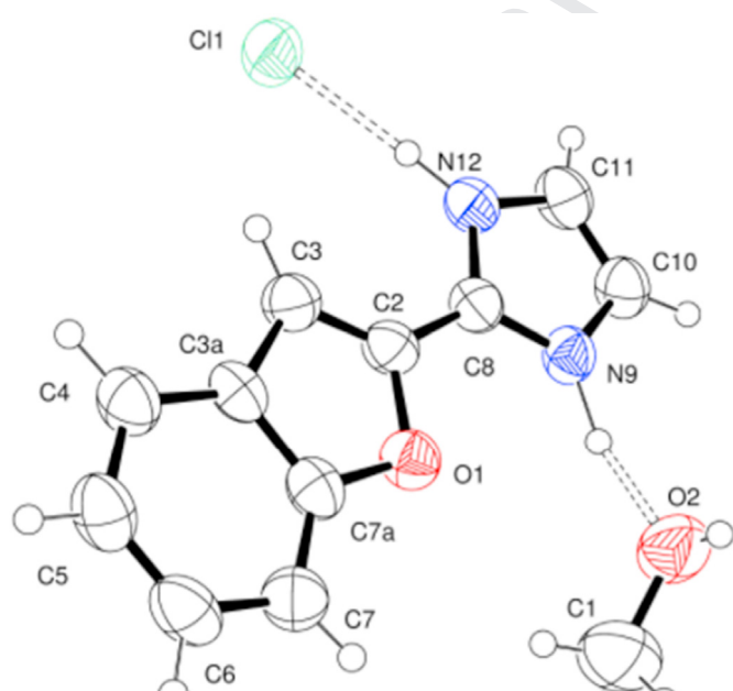
Fig. 8. X-ray structure of LSL60101.
