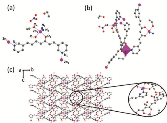
Fig. 5 Crystal structure of 4: (a) Representation of the coordination sphere of a \text{Zn}^{\text{II}} centre and the coordination mode of 3pyCCMoid; (b) picture of the connection of two neighbouring CCMoids; (c) 3D structure with molecules of the solvent and magnification of their disposition in the cavity. (Zn, pink; C, grey; O, red; N, blue; H atoms are omitted for clarity).
