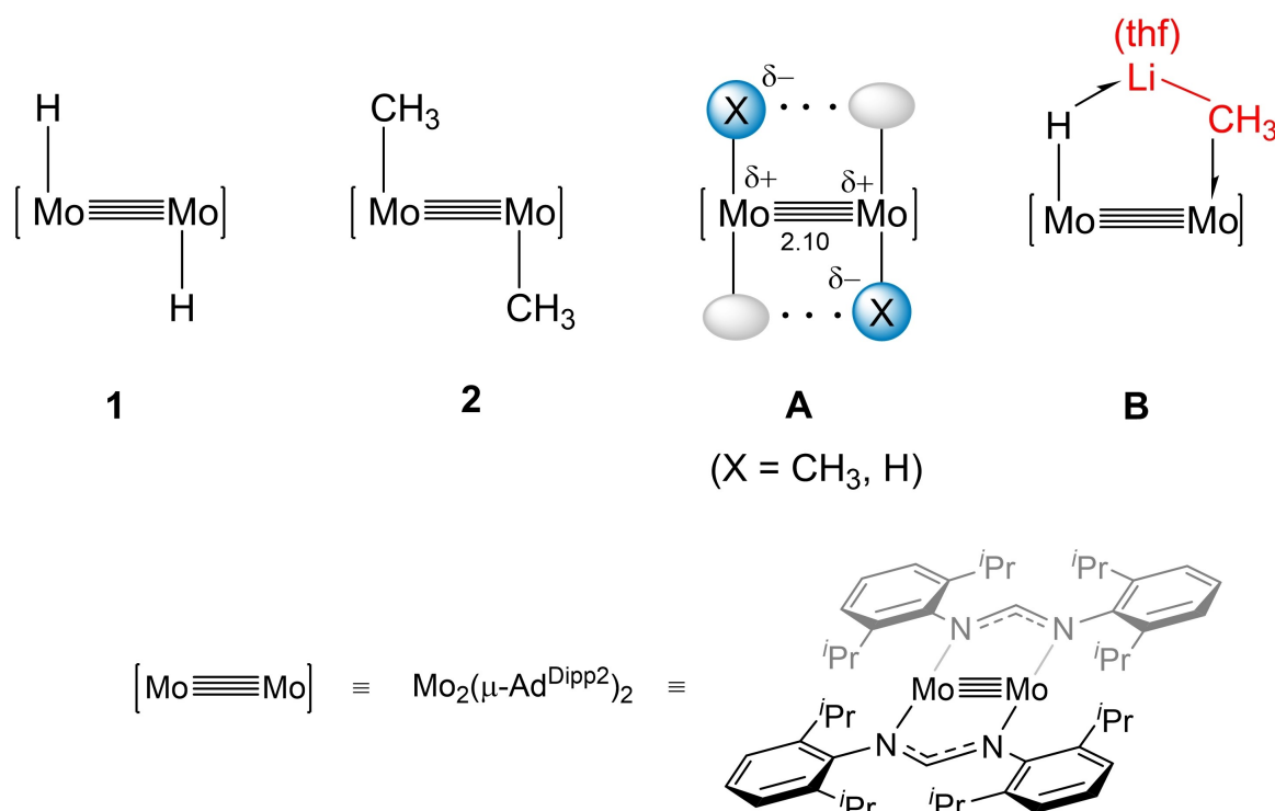
Figure 1. Simplified drawings of the structure of complexes [\text{Mo}_2(\text{X})_2(\mu\text{-Ad}^{\text{Dipp}2})_2] (X = H, 1 ; CH 3 , 2 ). Representation A highlights the bifunctional Lewis base/Lewis acid behavior, and potential cooperative effects between the Mo–X moieties (ellipsoids symbolize vacant coordination sites). B illustrates the multicenter structure resulting from the coordination of (thf)LiCH 3 to a (H)Mo≡Mo unit. In this and following figures and schemes, [\text{Mo}\equiv\text{Mo}] represents the fragment [\text{Mo}_2(\mu\text{-Ad}^{\text{Dipp}2})_2] .
