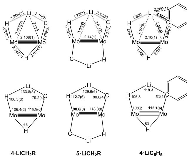
Figure 4. Average bond lengths and angles (in Å and °) for the Mo 2 Li(C)(H) metallacycles of studied complexes. The thick gray lines indicate distances significantly longer than the covalent radii sums. Numbers in boldface highlight the most relevant differences with the corresponding bonding parameters in 4 ·LiCH 2 R. The values shown are averages of experimental and calculated values, except for those parameters involving the hydride atom close to the Li atom, for which only calculated data were used.
