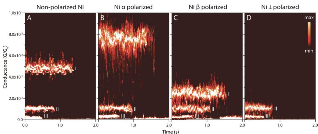
Figure 4. 2D conductance maps were obtained by accumulating hundreds of background-subtracted blinks set at a common time origin for [Cu( DPP )] under (A) non-polarized, (B) \alpha -Ni tip, (C) \beta -Ni-tip and (D) perpendicularly magnetized electrodes. The 2D maps color counts were normalized versus the total number of counts. Applied voltage bias and initial setpoint currents were -7.5 mV and 7 nA, respectively.
