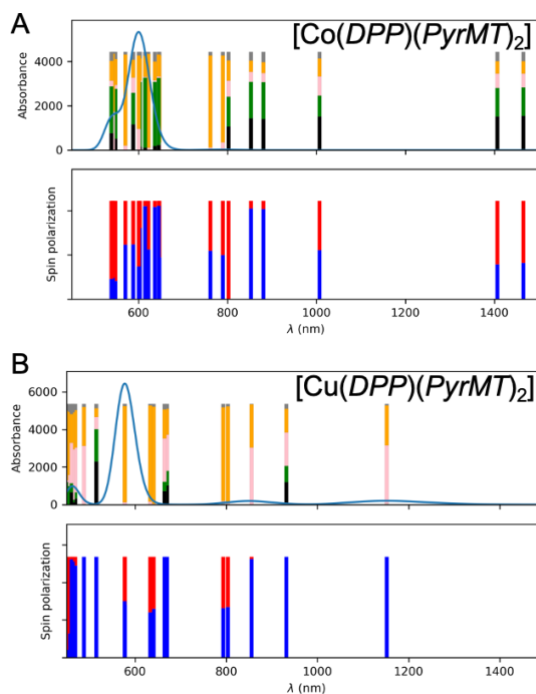
Figure 7. TD-DFT spectrum (TPSSH functional and def2-TZVP basis set) for [\text{Co}(\text{DPP})]/\text{PyrMT} (A) and [\text{Cu}(\text{DPP})]/\text{PyrMT} (B). The blue curve corresponds to the calculated spectrum. Each transition is represented in the absorbance graph by a vertical line, where colors indicate their transition composition (metal-metal: black; metal-ligand: green; ligand-metal: pink; ligand-ligand: orange). The spin polarization of the transition is represented in red: spin up, blue: spin down. Results for the four- and five-coordinated models are presented in SI section S5.
