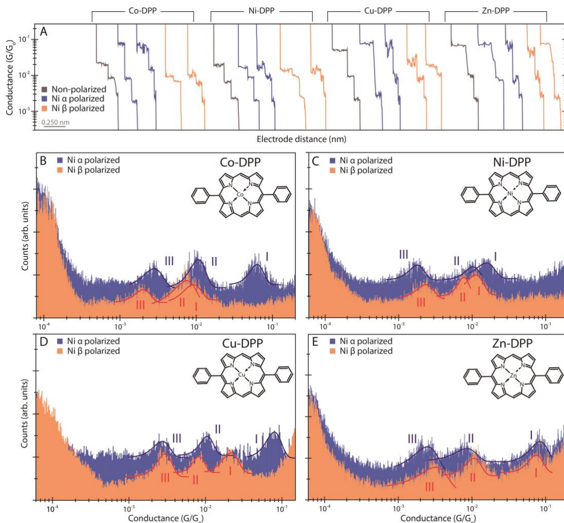
Figure 2. (a) Representative individual current traces displaying plateau features used to build the 1D histograms in B-E. (B-E) Single-molecule conductance 1D semi-log histograms for the metal porphyrins (labelled and represented in the figure) bridging between Au and both \alpha (blue) and \beta (orange) magnetically polarized Ni tips using PyrMT as anchoring ligand. Electrons are injected from the Au substrate to the Ni tip. All conductance values have been extracted from Gaussian fits of the peaks. Counts have been normalized versus the total amount of traces. All histograms display three peaks named conductance features I, II and III. The applied bias was set to -7.5 mV (see equivalent figures for positive bias in Fig. S1.6).
