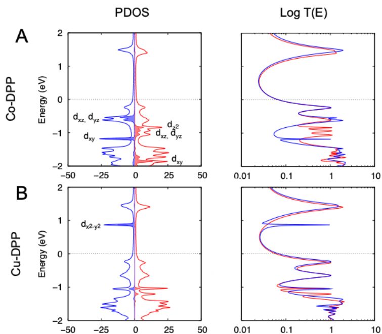
Figure 6. DFT calculated spin-resolved projected density of states (PDOS) and transmission spectra ( T(E) ) for the conductance feature I of the [\text{Co}(\text{DPP})]/\text{PyrMT} (A) and [\text{Cu}(\text{DPP})]/\text{PyrMT} (B) systems obtained with the Siesta and Gollum codes using PBE functional. Filled curves in the PDOS graphs denotes transition metal energy levels. Red and blue colors correspond to the alpha and beta spin contributions, respectively.
