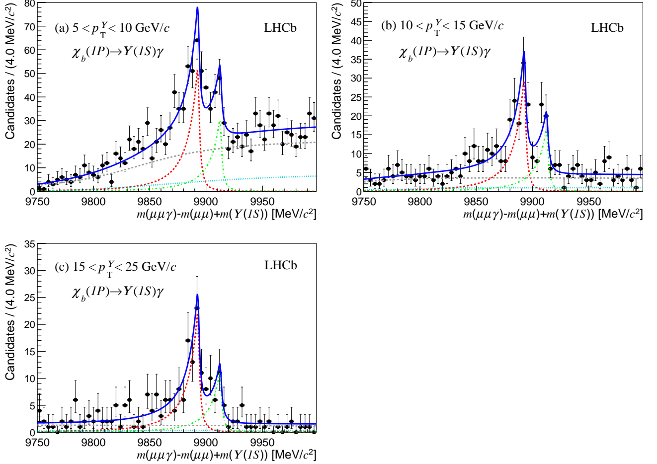
Figure 3: Distribution of m^*(\mu^+\mu^-\gamma) \equiv m(\mu^+\mu^-\gamma) - m(\mu^+\mu^-) + m(\mathcal{Y}) for \chi_b(1P) candidates with fit projections overlaid for each of the three ranges in p_T^{\mathcal{Y}} : (a) 5–10 GeV/c, (b) 10–15 GeV/c and (c) 15–25 GeV/c. The cyan dotted line shows the non- \mathcal{Y} background, the grey dashed line shows the combinatorial background, the red dashed line the \chi_{b1} contribution, the green dash-dotted line the \chi_{b2} contribution and the blue full line the sum of all these contributions.
