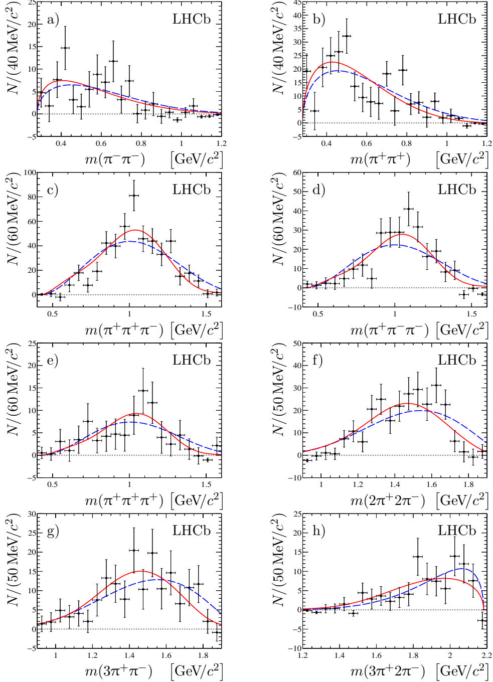
Figure 4: Distributions of (a) \pi^-\pi^- , (b) \pi^+\pi^+ , (c) \pi^+\pi^+\pi^- , (d) \pi^+\pi^-\pi^- , (e) \pi^+\pi^+\pi^+ , (f) 2\pi^+2\pi^- , (g) 3\pi^+\pi^- and (h) 3\pi^+2\pi^- masses in the B^+ \rightarrow J/\psi 3\pi^+2\pi^- decay. The prediction from the factorisation-based model is shown by solid (red) lines, and the expectation from the phase-space model is shown by dashed (blue) lines.
