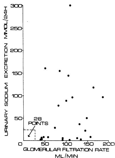
Fig. 1 Relationship between sodium excretion and glomerular filtration rate in the complete series.
