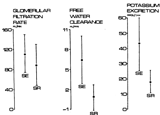
Fig. 2 Comparison of glomerular filtration rate, free water clearance, and potassium excretion in patients with glomerular filtration rate > 40 ml/min. Values for potassium excretion in patients with arterial pH > 7.50 are not included (SE—sodium excretors, SR—sodium retainers; mean values with standard deviations shown)
