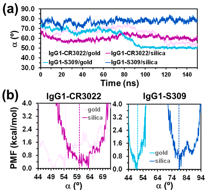
Fig. 2. (a) Temporal evolution of \alpha along the cMD trajectories. (b) PMF profiles of \alpha as derived from the aMD samplings for IgG1-CR3022 and IgG1-S309 tethered to the silica and gold surface. The dashed lines in the PMF profiles, which display the region with \Delta G \leq 4.0 kcal/mol, indicate the position of the average from cMD.
