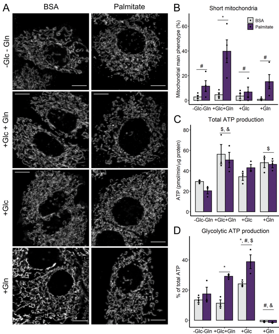
Fig. 4. Palmitate-induced metabolic shift requires glucose, but not mitochondrial network fragmentation - Cells were incubated with palmitate/BSA (0.2 mM/0.25%) for 6 h in media without glucose nor glutamine (-Glc-Gln), or in the presence of glucose and glutamine (Glc + Gln), only glucose (Glc), or only glutamine (Gln). Live mitochondrial morphology was evaluated by confocal microscopy at 6 h after 50 nM Mitotracker Deep Red loading (A). Mitochondrial network morphology was classified as described in the Methods section (B). ATP production was calculated as described in the Methods section (C-D). * = p < 0.05 or ** = p < 0.01 ; # p < 0.05 vs. -Glc-Gln; # = p < 0.05 vs. Glc + Gln. Two-way ANOVA followed by Tukey's post-test. Bar plots are means \pm SD. Filled circles represent independent experiments. Scale bar = 10 \mu m. (For interpretation of the references to color in this figure legend, the reader is referred to the Web version of this article.)
