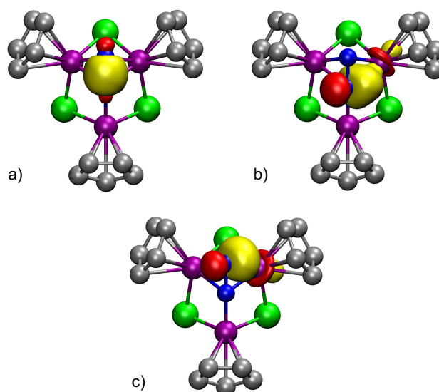
Figure 5. Compound 6 NBO orbitals within the \text{N}_2 unit: a) N–N bond; b) and c) Ti3–N1 and Ti3–N5 bonds (analogous NBO orbitals for Ti2–N1 and Ti2–N5 bonds were also found). Methyl groups of the \eta^5\text{-C}_5\text{Me}_5 ligands are omitted for clarity.
