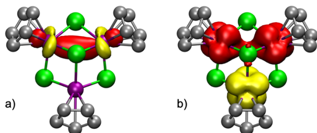
Figure 2. Computed a) half full Ti2–Ti3 alpha bonding orbital and b) spin density for compound 3 . Methyl groups of the \eta^5 -C 5 Me 5 ligands are omitted for clarity.
