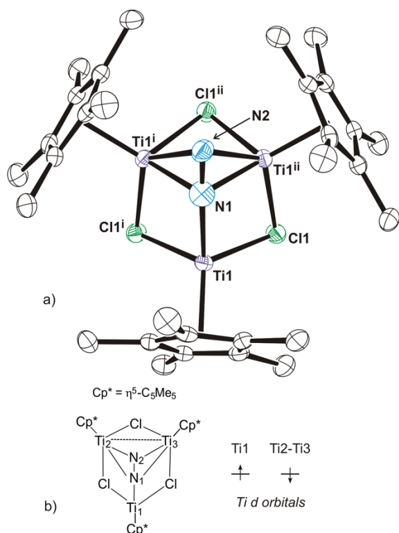
Figure 3. a) Perspective view of complex 6 (thermal ellipsoids at the 50% probability level). Hydrogen atoms of the \eta^5\text{-C}_5\text{Me}_5 ligands are omitted for clarity. Selected lengths ( \text{\AA} ) and angles ( ^{\circ} ): Ti–Ti 2.936(1) , Ti–Cl av. 2.395(4) , Ti(1)–N(1) 2.017(3) , Ti(1)–N(2) 2.146(9) , Ti(1)–N(2) 2.099(10) , N(1)–N(2) 1.099(9) , Cl–Ti–Cl 95.9(1) , N(1)–Ti–Cl av. 95.5(1) , Ti–Cl–Ti 75.6(1) , Ti–N(1)–Ti 93.4(2) , Ti–N(1)–N(2) 170.2(7) , Ti–N(2)–Ti 87.5(4) . Symmetry code: (i) 1 - y, x - y, z ; (ii) 1 - x + y, 1 - x, z . b) Most stable computed singlet electronic structure for compound 6 .
