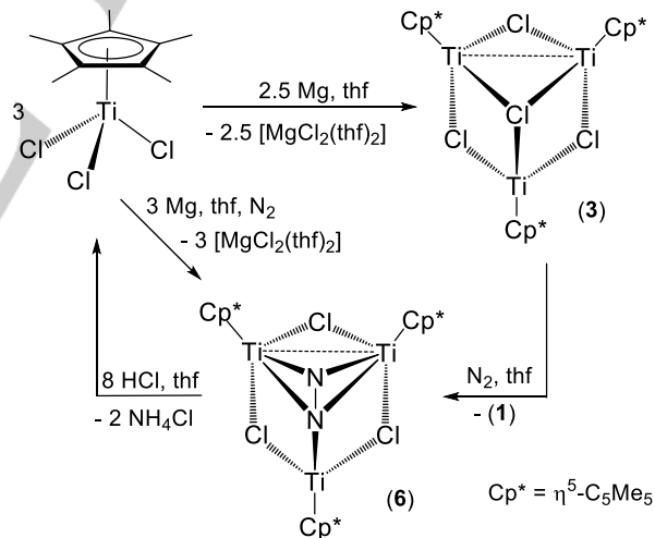
Scheme 2. Reaction of [TiCp*Cl 3 ] with magnesium under N 2 atmosphere.
