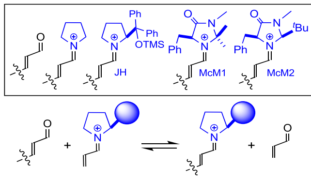
Scheme 2. Main Species and Equilibria Calculated
