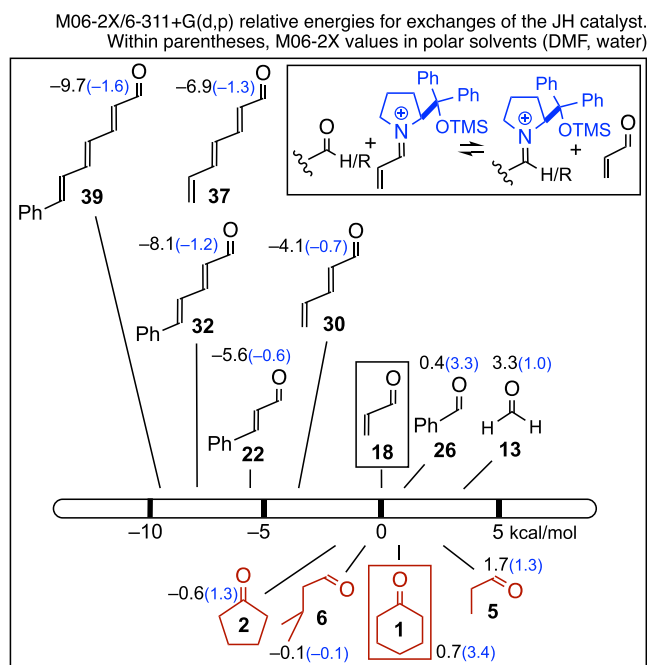
Figure 2. Relative energies in kcal/mol for the exchange equilibria between JH-derived iminium ions and carbonyl compounds.
