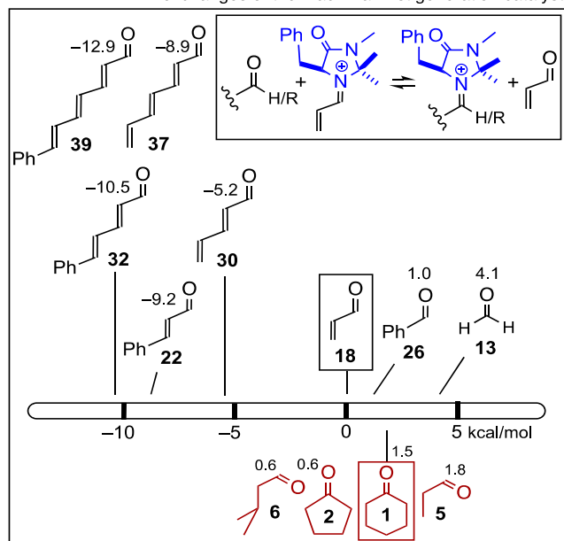
M06-2X/6-311+G(d,p)-based relative energies for representative exchanges of the MacMillan-1st generation catalyst)
