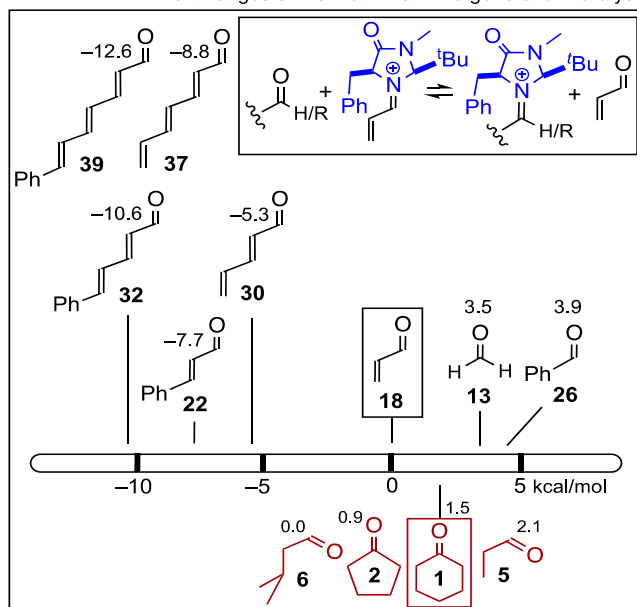
Figure 3. Relative energies in kcal/mol for the equilibria between carbonyl compounds and MacMillan-type iminium ions.
