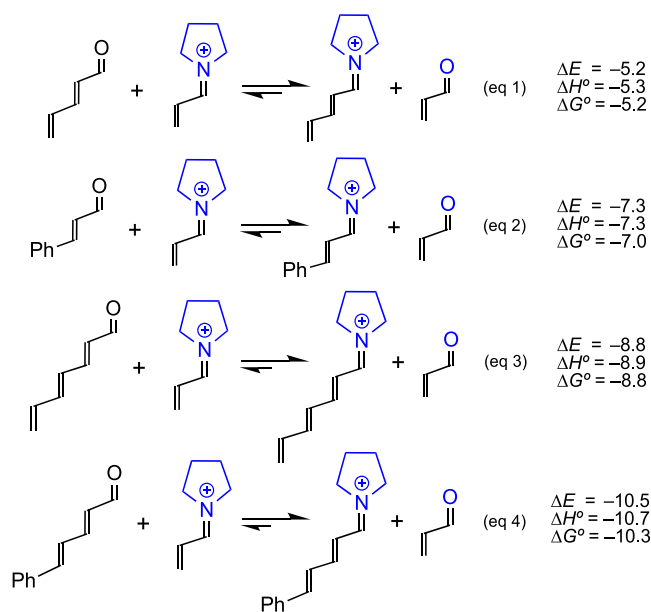
Scheme 3. Exchange of Pyrrolidine between Enals, Dienals, and Trienals and Their Iminium Ions a
