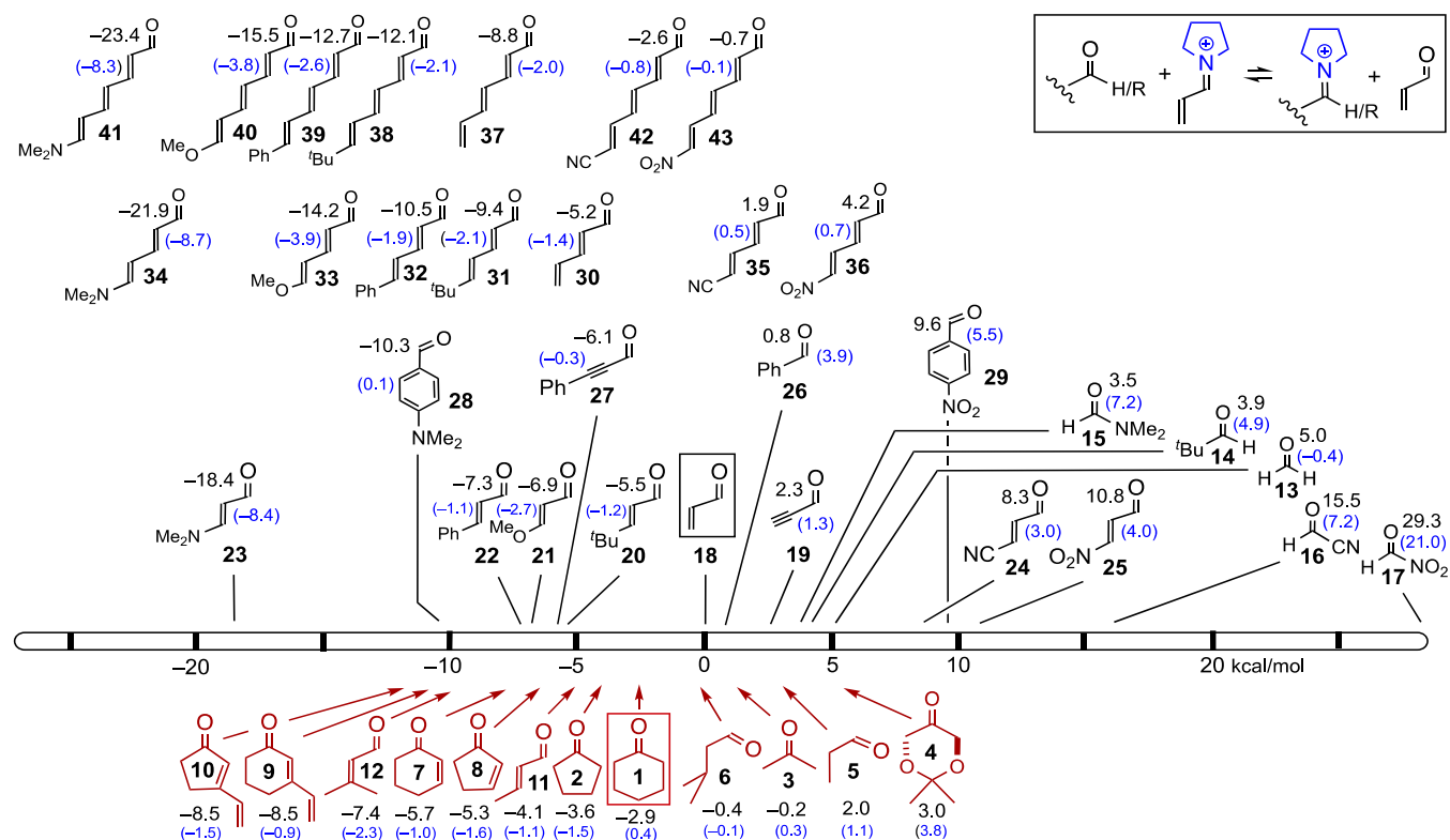
Figure 1. Relative energies for equilibria between pyrrolidine-derived iminium ions and carbonyl compounds.
