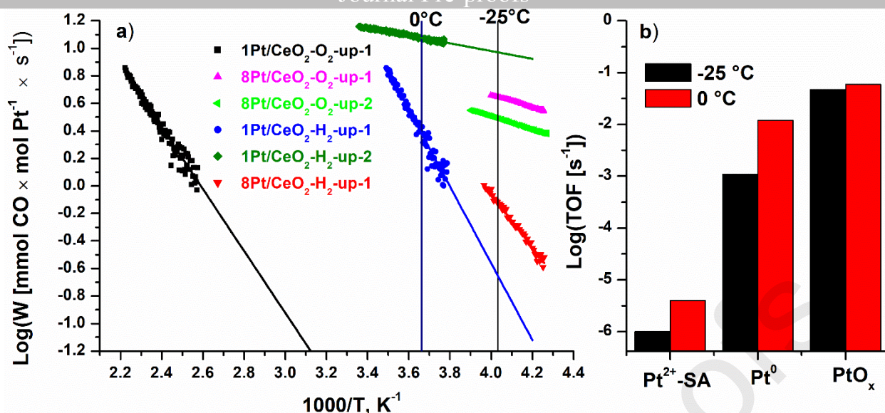
Fig. 3. a) Arrhenius dependences of the CO oxidation reaction rate W (decimal logarithmic W versus 1/T ) using the 1Pt/CeO 2 -O 2 , 1Pt/CeO 2 -H 2 , 8Pt/CeO 2 -O 2 and 8Pt/CeO 2 -H 2 catalysts obtained by their heating treatments up-1 and up-2. Straight lines for the 1Pt/CeO 2 catalysts indicate extrapolated values; b) \text{Log}(\text{TOF}) at -25 and 0^\circ\text{C} for the 1Pt/CeO 2 catalysts O 2 -up-1, H 2 -up-1 and H 2 -up-2 containing Pt 2+ -SA, Pt 0 , and PtO x active forms after pre-treatments by O 2 , H 2 , and the CO+O 2 reaction mixture, respectively.
