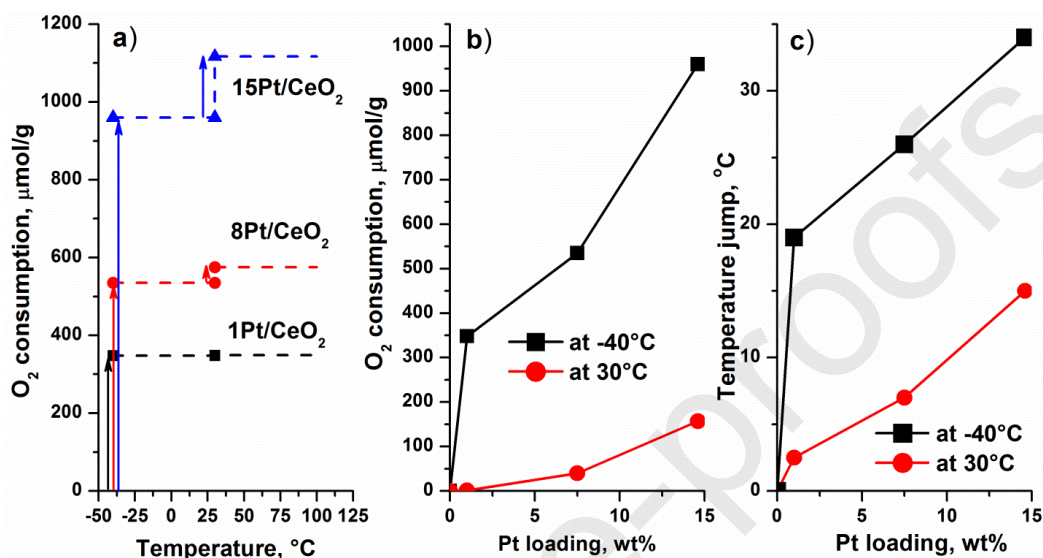
Fig. 5. a) Temperature dependence of the \text{O}_2 amount consumed for oxidizing the catalysts 1Pt/CeO 2 -Red, 8Pt/CeO 2 -Red and 15Pt/CeO 2 -Red upon admission of the reaction mixture; b) Dependences of the \text{O}_2 consumption at -40^\circ\text{C} and in the interval 25 - 50^\circ\text{C} on Pt loading in the catalysts; c) Temperature jump (response) of the reduced catalysts upon \text{CO}+\text{O}_2 admission followed by heating of the reactor. These data were calculated from the time dependencies of the \text{O}_2 consumption and of the \text{CO}_2 evolution shown in Fig. S3.
