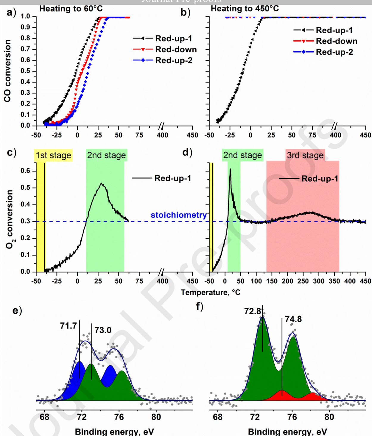
Fig. 6. Temperature dependences of CO conversion (a, b) and O 2 conversion (c, d) for the 8Pt/CeO 2 -Red catalyst during TPR-CO-O 2 upon heating to 60°C (a, c) and 450°C (b, d); curve-fitted Pt 4f XPS spectra of the 8Pt/CeO 2 -Red sample after heating to 60°C (e) and 450°C (f), see color coding in Fig. 2a.
