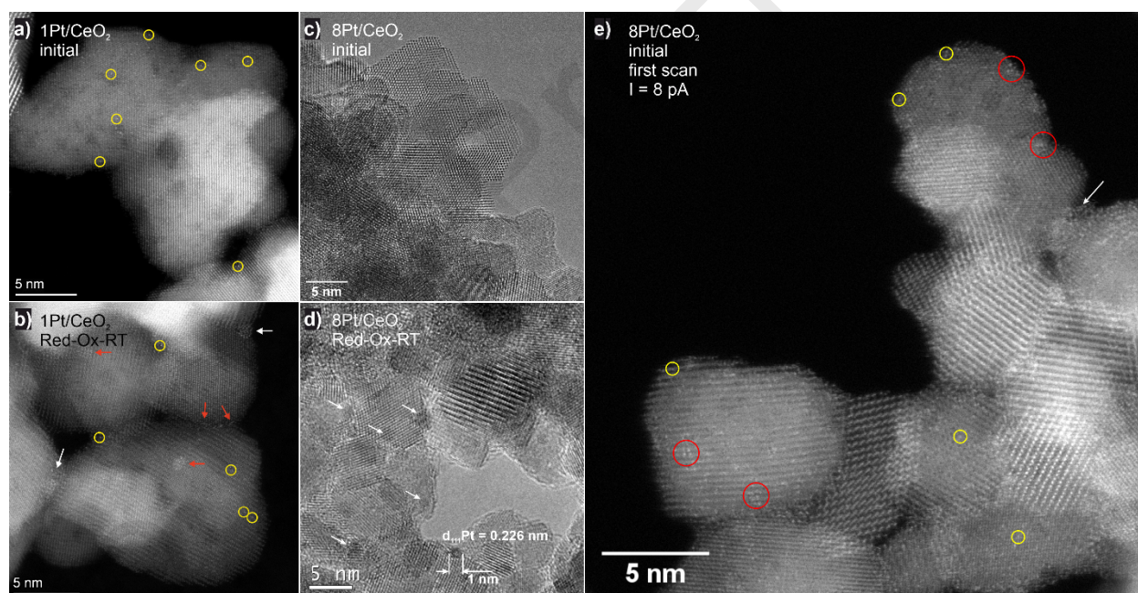
Fig. 8. (a) HAADF-STEM image of the initial 1Pt/CeO 2 catalyst; (b) HAADF-STEM image of the 1Pt/CeO 2 catalyst after Red-Ox-RT treatment; (c) HRTEM image of initial 8Pt/CeO 2 with no evidence for Pt clusters; HRTEM image of 8Pt/CeO 2 catalyst after Red-Ox-RT treatment showing numerous Pt clusters; (e) HAADF-STEM image of the initial 8Pt/CeO 2 catalyst: first scan with a low beam current, where most of platinum is present in atomically-dispersed state. Yellow circles – single Pt atoms, red circles – several agglomerated Pt atoms, red arrows – flat Pt species consisting of several Pt atoms, white arrows – Pt clusters.
