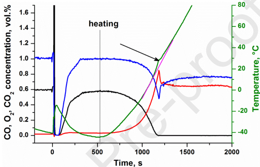
Fig. 4. Evolution with time of CO, CO 2 and O 2 concentrations and temperature upon switching on feeding of the reaction mixture to the reactor (zero on the time axes) for the reduced 8Pt/CeO 2 -Red catalyst. Vertical lines designated as “heating” show the onset of catalyst heating started at achieving a quasi-stationary regime after the reactants admission at low temperature. Arrows indicate the temperature maximum due to the catalyst overheating; the expected curve without the overheating is shown in pink.
