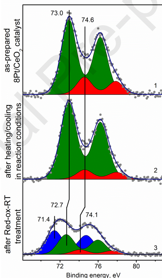
Fig. 7. Fitted Pt4f spectra of the 8Pt/CeO 2 catalyst: (1) as-prepared; (2) after two heating/cooling runs of CO+O 2 reaction to 450°C (see also Figs. 1, 2, and 6); (3) after Red-Ox-RT treatment. Integrated Pt 0 /Pt δ+ , Pt 2+ and Pt 4+ peaks are colored in blue, green and red, respectively.
