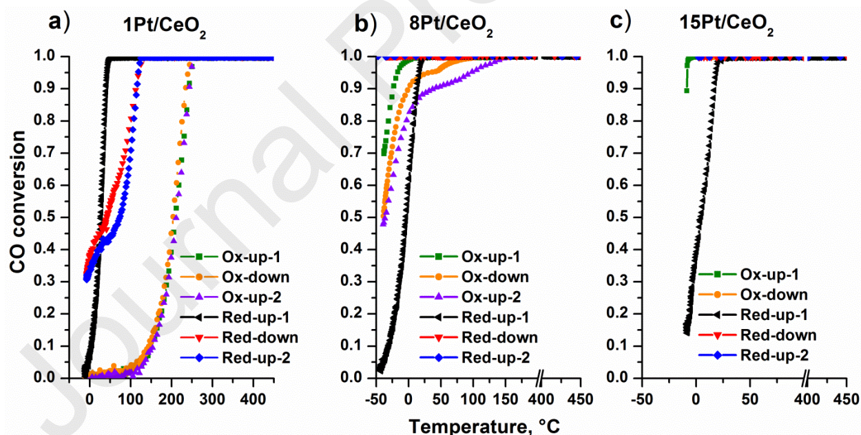
Fig. 1. Temperature dependences of CO conversion for (a) 1Pt/CeO 2 , (b) 8Pt/CeO 2 and (c) 15Pt/CeO 2 catalysts after pretreatments in 20%O 2 /He at 450°C for 2 hours (Ox) and in 40%H 2 /He at 300°C for 2 hours (Red) in the temperature-programmed regime in CO oxidation during the heating up-1 , the cooling down and the second heating up-2 .
