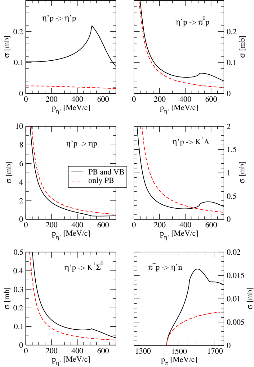
FIG. 3: Elastic and inelastic \eta'p cross sections, as functions of the \eta' momentum in the lab frame, together with the cross section of the reaction \pi^-p \rightarrow \eta'n as function of the pion momentum. Dashed lines correspond to the results obtained with the standard model that considers only the coupling to PB states, while solid lines also contain the coupling to the VB channels.
