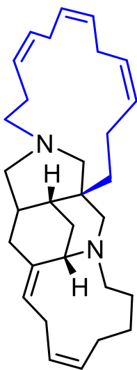
Madangamine A
