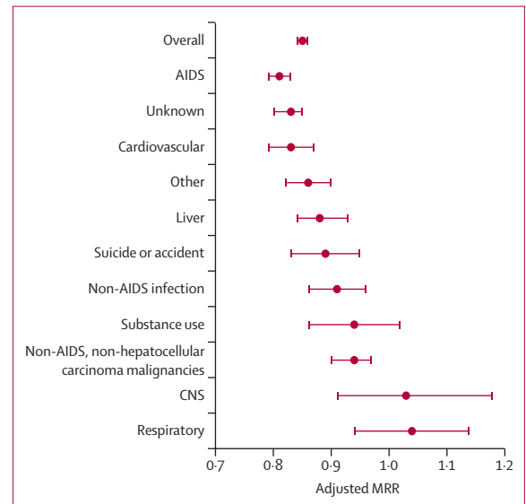
Figure 3: Adjusted* cause-specific MRRs per period (1996–99, 2000–03, 2004–07, 2008–11, 2012–15, 2016–2020†), with 95% CIs CNS category includes Parkinson's and Alzheimer's disease. MRR=mortality rate ratio. *Adjusted for CD4 cell count category and age group at the start of the period, whether the participant was ART-naïve when starting the period, and cohort. †Calendar year period is modelled as a continuous variable; the MRRs can be interpreted as a per-period decrease.
