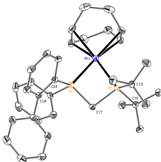
Fig. 7 ORTEP plot of RhBiphzBu with ellipsoids drawn at 50% probability level. Hydrogen atoms and the tetrafluoroborate anion have been omitted for clarity. Selected distances (Å) and angles (°): Rh1–P1 2.2861(7), Rh1–P2 2.3356(7), P1–C17 1.837(3), P2–C17 1.857(3), P1–Rh1–P2 72.35(2).
