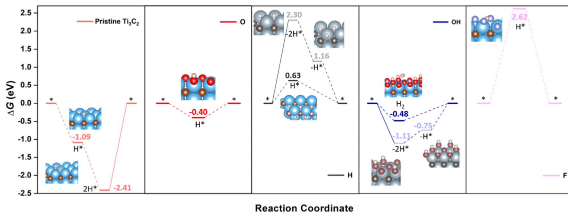
Fig. 4 Gibbs free energy, \Delta G , diagram of the HER on pristine or fully -\text{O} , -\text{OH} , -\text{F} , or -\text{H} terminated \text{Ti}_3\text{C}_2 (0001) surface under standard working conditions. Solid lines represent the chemical step of the as-generated \text{H}_2 desorption, while dashed lines represent the electrochemical steps of proton coupled electron transfer (PCET). Inset images are side or eagle-eye views of the reaction intermediates, except for the \text{H}^* state on -\text{H} termination, which depicts a top view to better observe the \text{H}^* allocation on a surface empty \text{H}_\text{C} site. Color coding as in Fig. 1, plus H, O, and F atoms are shown as white, red, and violet spheres. Preferred reaction mechanism and associated images are shown with bright coloring, while shadowed colors and images refer to other, non-preferred mechanisms.
