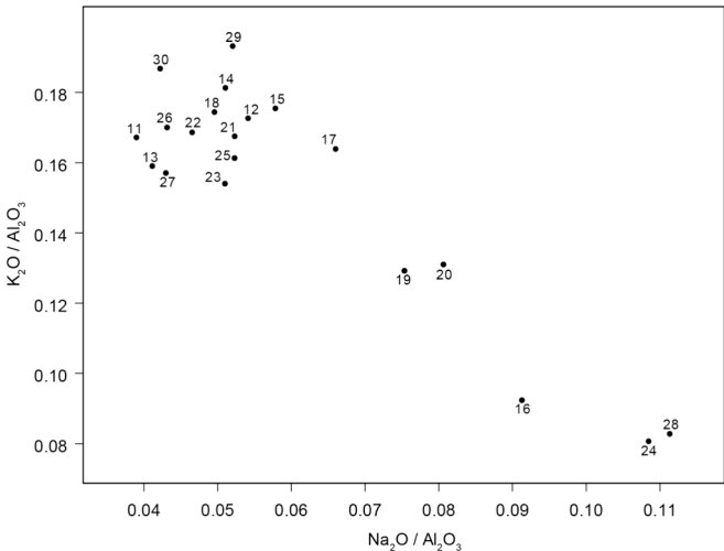
Fig. 7. Binary variation diagram of Na 2 O/Al 2 O 3 vs K 2 O/Al 2 O 3 for the ‘Kuass ware’ samples analysed from Málaga, showing the presence of five samples with higher Na 2 O and lower K 2 O than the rest of the data set. For each sample the MAL19/- prefix was removed to simplify the reading.
