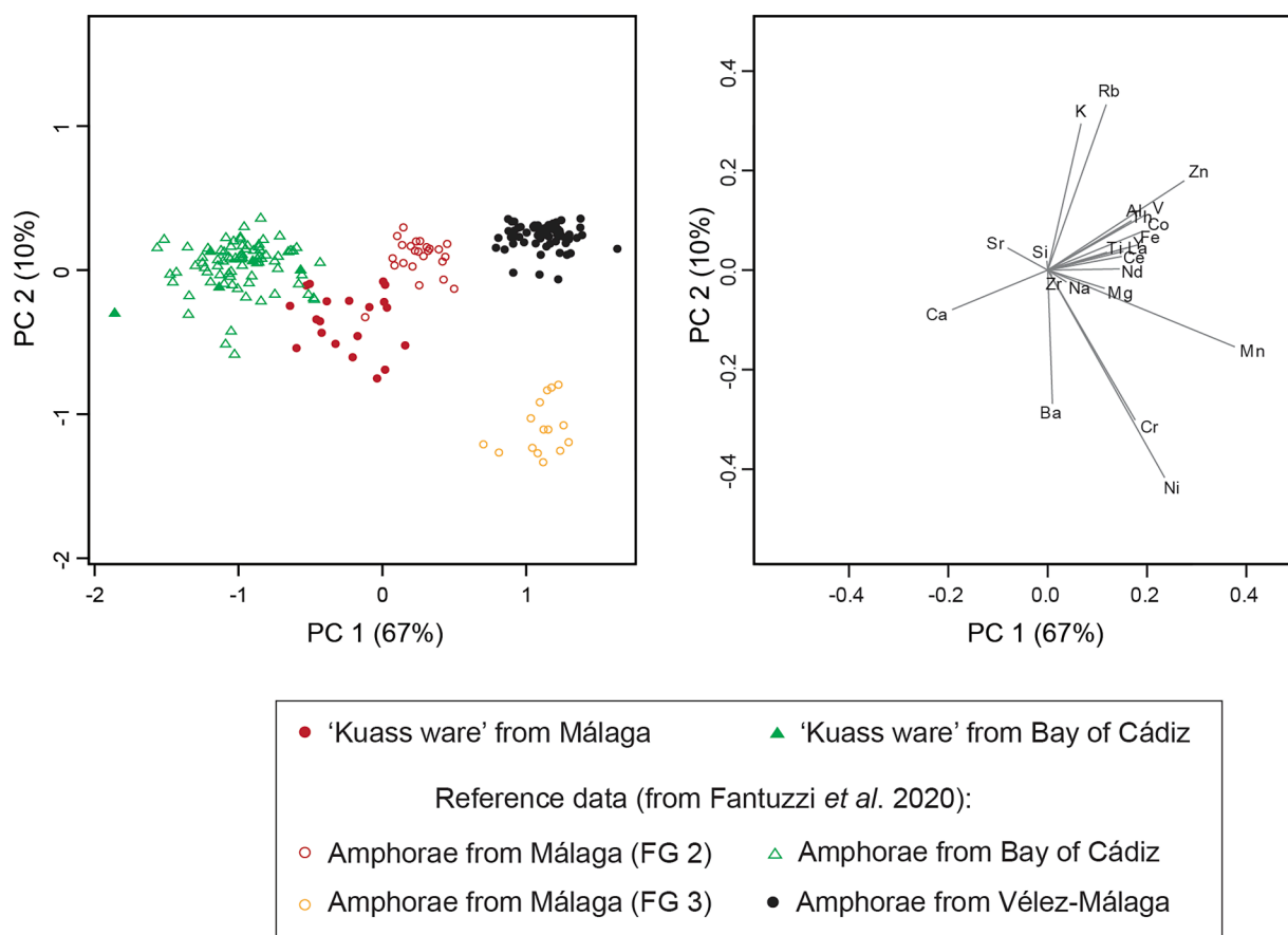
Fig. 10. PCA of the log transformed elemental data (WD-XRF) for the 25 'Kuass ware' samples compared to previously published data by Fantuzzi et al. (2020) for Punic amphorae and clay samples. The PCA was performed on the log transformed subcomposition Na, Mg, Al, Si, K, Ca, Ti, Fe, V, Cr, Mn, Co, Ni, Zn, Rb, Sr, Y, Zr, Ba, La, Ce, Nd, and Th (P, Pb, and Cu were excluded to avoid possible contamination problems). (a) Biplot PC1 vs PC2. (b) Projections of elemental loadings.
