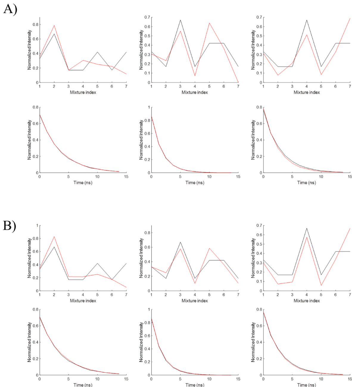
Fig. 6. ATTO dataset (15 sampling points). A) Top panel, concentration profiles recovered by PARAFAC-ALS for PowerSlicing (red) and expected concentration profiles (black). Bottom panel, pure fluorescence decays recovered by PARAFAC-ALS for PowerSlicing (red) and expected pure fluorescence decays (black). B) Top panel, concentration profiles recovered by PARAFAC-ALS for Kernelizing (red) and expected concentration profiles (black). Bottom panel, pure fluorescence decays recovered by PARAFAC-ALS for Kernelizing (red) and expected pure fluorescence decays (black). (For interpretation of the references to colour in this figure legend, the reader is referred to the Web version of this article.)
