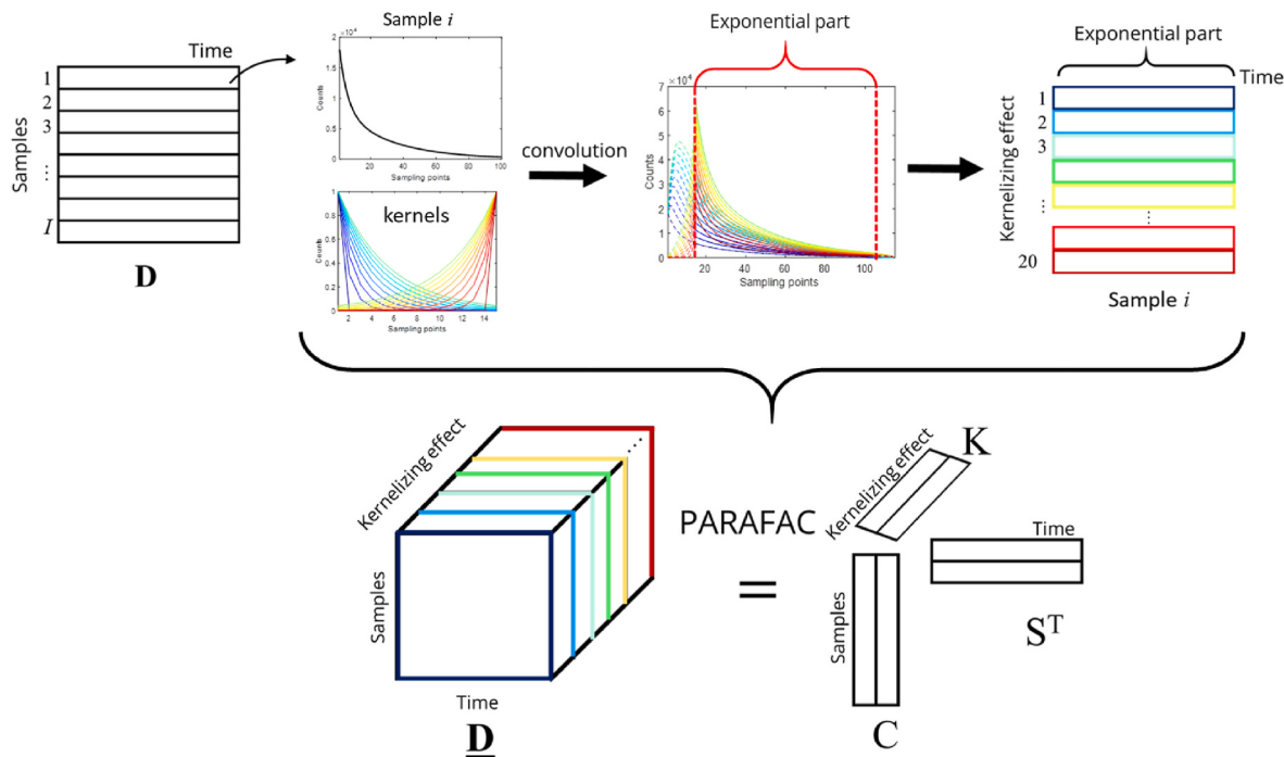
Fig. 3. Schematic representation of the Kernelizing approach. Each decay of the matrix \mathbf{D} is convolved individually with a set of different kernels. Then, only the exponential parts of the resulting curves are kept and gathered into a matrix. After convolving every sample with the aforementioned kernels, a trilinear data array \mathbf{D} can be built and subsequently analyzed by PARAFAC-ALS.
