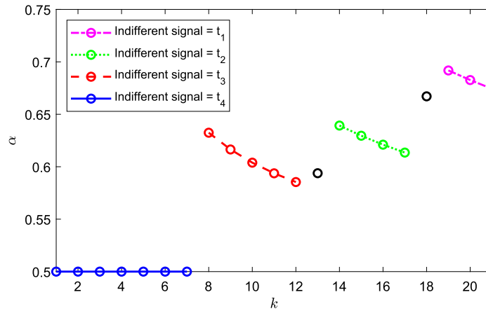
Fig. 1. The function \alpha_M(k, \mathcal{N}) . Parameters: p = 1/2 , \mathcal{N} = 21 , r_F = (1/8, 3/16, 1/4, 7/16) , r_F = (1/4, 1/4, 1/4, 1/4) .
