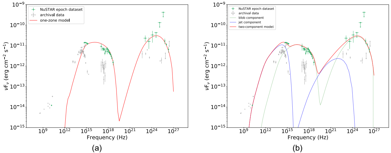
Figure 8. Broad-band SED and modelled spectra for TXS 1515–273. The SED has been modelled considering the VLBA SED point in the radio band, KVA, Swift , and NuSTAR SED points in the optical and X-ray energy band and the Fermi -LAT and MAGIC SED points in the gamma-ray band, using a one-zone model (left) and a two-component model (right). Only Swift data simultaneous to NuSTAR observations were used. Coloured points represent observations in the different energy bands during the observations of 2019, grey points represent archival data. The red solid line represents the models, the green dotted line represents the blob emission and the blue dashed line represents the jet emission. Further details can be found in the text. For parameters, see Table 5.
