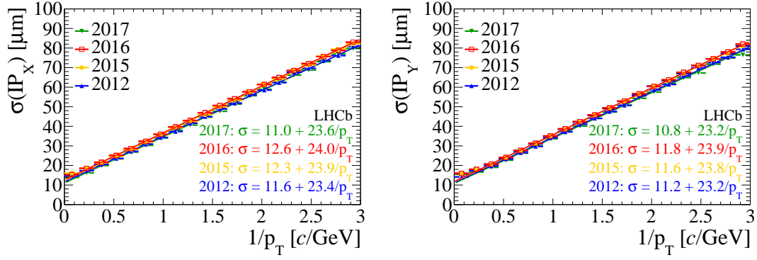
Figure 12. Resolution of the x (left) and y (right) components of the impact parameter comparing the 2012 (blue), 2015 (orange), 2016 (red) and 2017 (green) data-taking periods. The resolution as a function of p_T is given in the bottom right corner.
