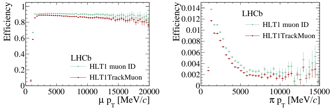
Figure 7. HLT1 muon identification efficiency for (left) muons from J/\psi \rightarrow \mu^+\mu^- decays and (right) pions from D^0 \rightarrow K^-\pi^+ decays. Green circles show only the identification efficiency (HLT1 Muon ID) while red squares show the efficiency of the additional trigger line (named HLT1TrackMuon) requirements (see text).
