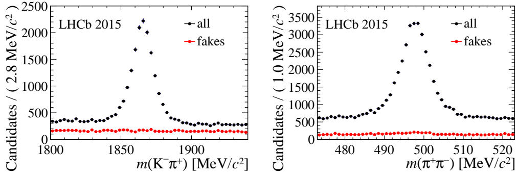
Figure 9. Performance of the fake-track classifier on (left) D \rightarrow K^- \pi^+ and (right) K_s^0 \rightarrow \pi^- \pi^+ decays. For these plots, the clones have been removed.
