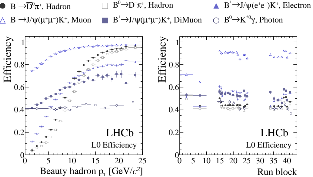
Figure 21. Efficiencies of the L0 trigger lines in Run 2 data for b -hadron decays. The left plot shows the efficiency as a function of the hadron p_T , while the right plot shows the evolution of the efficiency as a function of the different trigger configurations used during data taking. The three blocks visible in the plot, separated by vertical gaps, correspond to the three years of data taking (2015–2017). The plotted L0 efficiency for each b -hadron is described in the legend above the plots.
