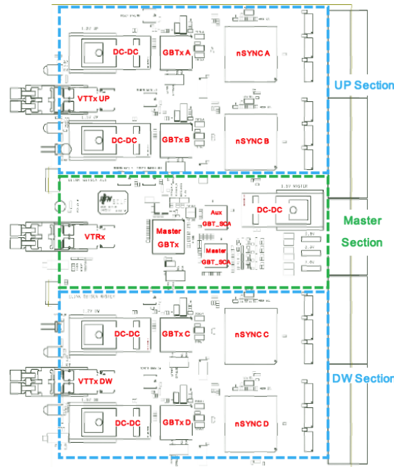
Figure 89. nNODE board layout.
