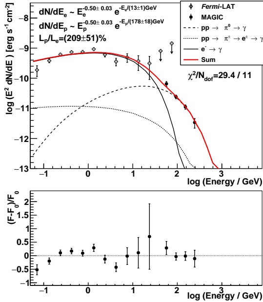
Supplementary Figure 2 Fit to the Fermi -LAT and MAGIC SED with a proton-electron model. The dashed line shows the gamma rays from the \pi^0 decay and the dotted line shows the inverse Compton contribution of the secondary e^\pm pairs produced in hadronic interactions. dN/dE_p and dN/dE_e report the shape of the proton and electron energy distributions obtained from the fit. The bottom panel shows the fit residuals. Errorbars represent 1-sigma statistical uncertainties in the data points.
