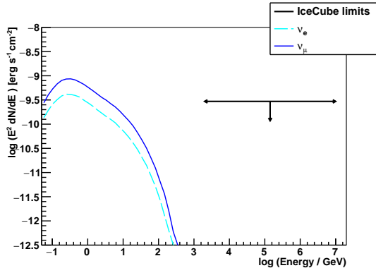
Supplementary Figure 1 Predicted neutrino emission ( \nu_e with cyan dashed line and \nu_\mu with solid blue line) associated to the proton model (see Fig. 3) compared with 90% C.L. limits obtained by the IceCube Collaboration [91].
