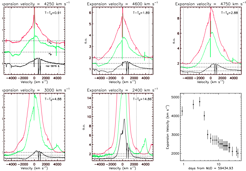
Extended Data Figure EDF 7 Example of H_{\alpha} , H_{\beta} and He I 5876 Å P-Cygni profiles used to determine the behavior of the expansion velocity of the expanding envelope (time after the outburst is given in the top right part of each panel). The bottom right panel shows the evolution of the velocity in time. Error bars represent 1-sigma statistical uncertainties in the data points.
