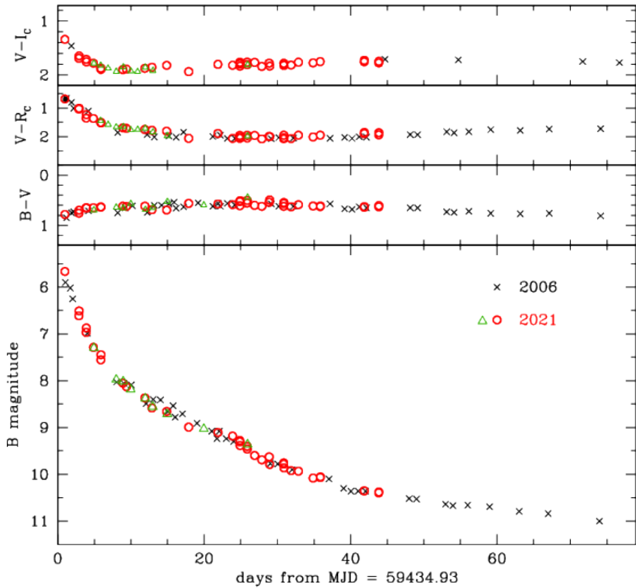
Extended Data Figure EDF 1 Optical B -band observed magnitude and the color index of RS Oph 2021 outburst from ANS (red circles) and TJO (green triangle) compared to that of 2006 eruption (black crosses, computed with respect to MJD of 53775.86, [69]). Top three panels show the color indices, while the bottom panel shows B magnitude evolution.
