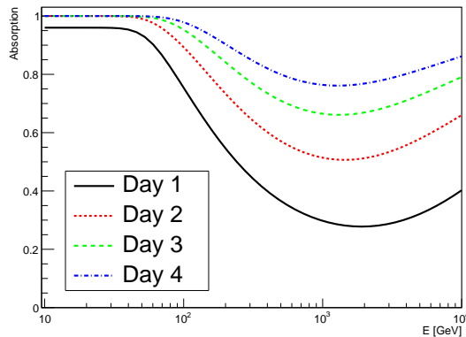
Extended Data Figure EDF 8 Absorption of the gamma-ray emission on the radiation field of the photosphere and collision with it. Assumed parameters: v_{sh} = 4500 \text{ km s}^{-1} , R_{ph} = 200 R_{\odot} . Temperature of the photosphere is T_{ph} = 10780 \text{ K} , 9490 \text{ K} , 8460 \text{ K} and 7680 \text{ K} for the time after the nova onset: 1 d (black solid), 2 d (red dotted), 3 d (green dashed), 4 d (blue dot-dashed) respectively.
