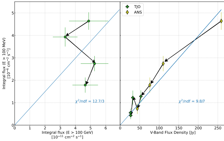
Extended Data Figure EDF 4 Comparison of the photon flux measured by Fermi -LAT above 100 MeV with the one measured by MAGIC above 100 GeV (left panel) and with that of the V-band obtained by ANS (right panel). Arrows show the sequence of the flux temporal evolution and the blue line shows the linear proportionality fit in both panels. Error bars represent 1-sigma statistical uncertainties in the data points.
