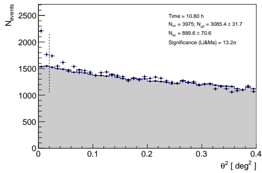
Extended Data Figure EDF 2 Distribution of the squared angular distance between the nominal source position and the reconstructed arrival direction of events (black crosses) and the estimated background (gray shaded area). Vertical dashed line represents the angular cut below which the number of background and excess events as well as the statistical significance of the detection are given (inset panel). Error bars represent 1-sigma statistical uncertainties in the data points.
