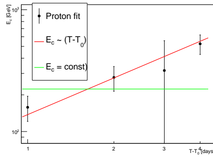
Extended Data Figure EDF 9 The maximum energy of protons obtained from the theoretical model fits to the daily gamma-ray emission (points) shown in Fig. 3. Red and green line show, respectively, the scenario of proportional increase and constant value of maximum energy. Error bars represent 1-sigma statistical uncertainties in the determination of the maximum energy of protons.
