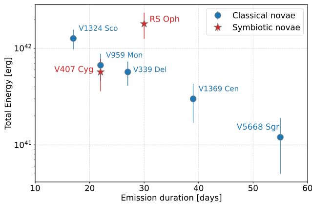
Fig. 4 Total energy vs duration of RS Oph 2021 outburst compared to that of the other novae detected by Fermi -LAT. Data taken from [14, 15, 68]. Errorbars represent 1-sigma statistical uncertainties in the data points.
