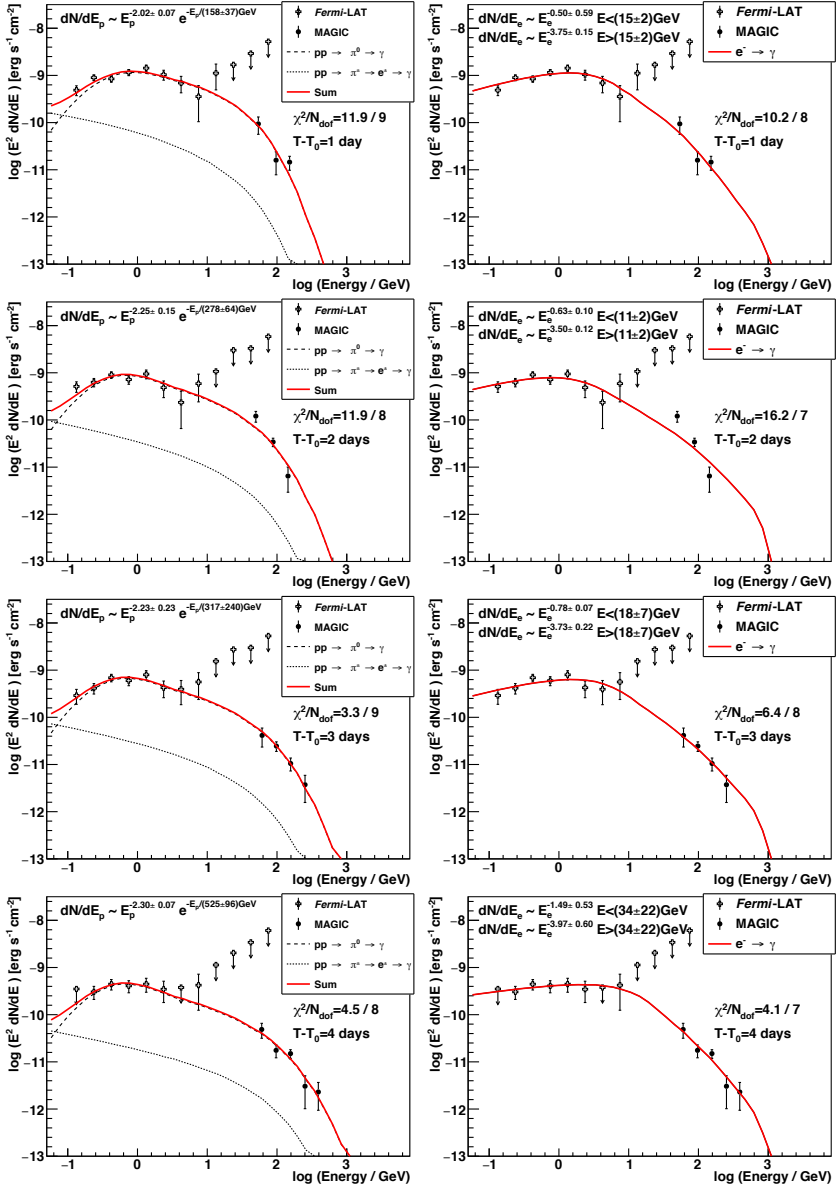
Extended Data Figure EDF 3 Modeling of daily emission in proton model (left panels) and electron model (right panels) for first, second, third and fourth day after the nova eruption (from top to bottom). The dashed line shows the gamma rays from the \pi^0 decay and the dotted line shows the inverse Compton contribution of the secondary e^\pm pairs produced in hadronic interactions. dN/dE_p and dN/dE_e report the shape of the proton and electron energy distributions obtained from the fit. The bottom panel shows the fit residuals. Error bars represent 1-sigma statistical uncertainties in the data points.
