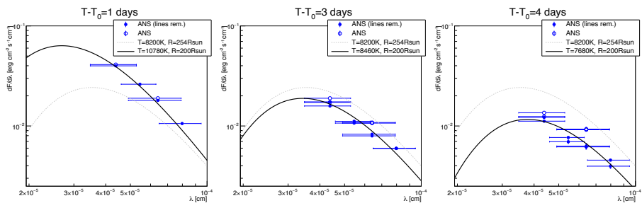
Extended Data Figure EDF 6 Optical photometry performed by ANS 1, 3, and 4 days (see the panel titles) after the outburst (blue empty markers) corrected for the Galactic absorption. Filled markers show the flux after subtraction of H\alpha and H\beta line contributions. The thick black lines show a black-body emission used in the modeling, while the dashed line shows for comparison the average 2006 spectral fit from [52] (with the photosphere radius corrected to the distance of 2.45 kpc). Horizontal error bars represent the bandwidth of the filters used.
