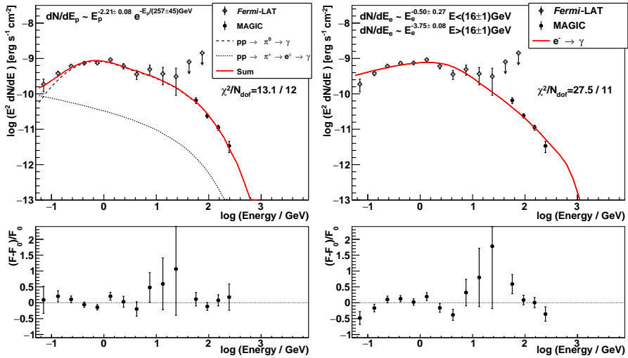
Fig. 3 Gamma-ray spectrum of RS Oph observed with Fermi -LAT (empty crosses) and MAGIC (filled circles) averaged over the first four days of the outburst, modeled within hadronic (left panel) or leptonic (right panel) scenario. The dashed line shows the gamma rays from the \pi^0 decay and the dotted line shows the inverse Compton contribution of the secondary e^\pm pairs produced in hadronic interactions. dN/dE_p and dN/dE_e report the shape of the proton and electron energy distributions obtained from the fit. The bottom panel shows the fit residuals. Errorbars represent 1-sigma statistical uncertainties in the data points.
