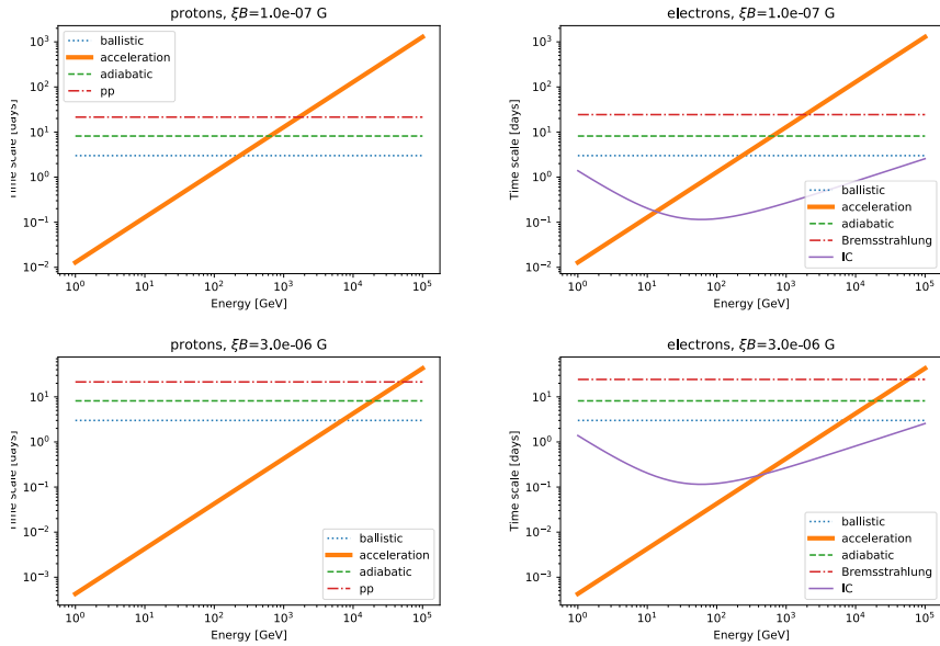
Extended Data Figure EDF 5 Cooling and acceleration time scale for protons (left panels) and electrons (right panels) for two values of \xi B parameter: 10^{-7} G (top panels) and 3 \times 10^{-6} G (bottom panels). Assumed parameters (see text for details): v_{sh} = 4500 \text{ km s}^{-1} , t = 3 \text{ d} , R_{ph} = 200 R_{\odot} , T_{ph} = 8460 \text{ K} , n_p = 6 \times 10^8 \text{ cm}^{-3} .
