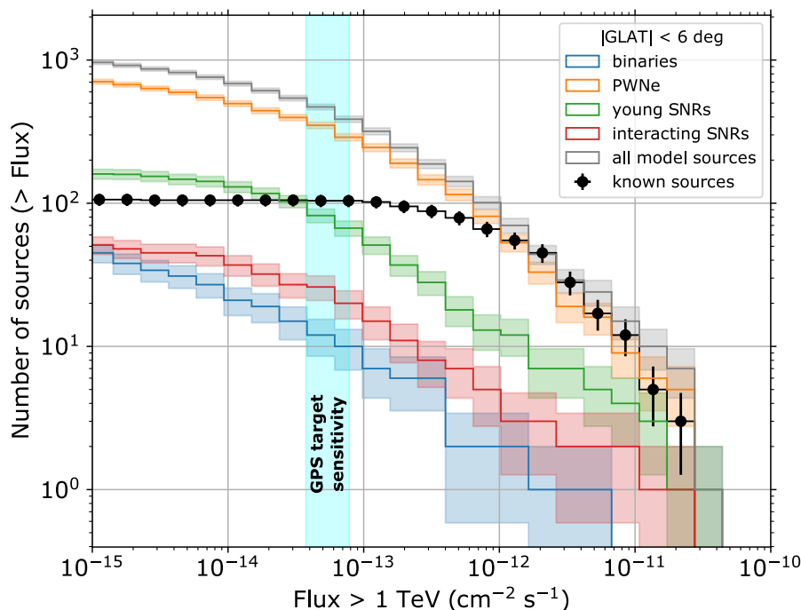
Figure 1. Cumulative number of sources for Galactic latitude < 6^\circ as a function of integral source flux above 1 TeV, showing known emitters and the synthetic source populations from our sky model for different source classes. For known emitters the vertical bars show the estimated Poisson fluctuations. The shaded blue vertical band shows the target sensitivity of the GPS defined in [24].
