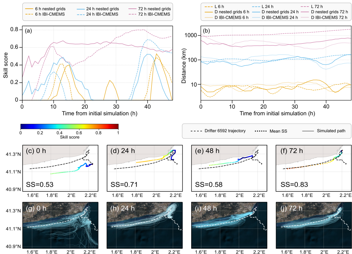
Figure 5. Lagrangian validation of LOCATE using data from drifter 6592 between 9 March and 14 March 2022 (maximum of 120 h) using the skill score test. Panel (a) illustrates the SS of the simulations at 6, 24 and 72 h forecast horizons using nested grids and the IBI-CMEMS grid. Panel (b) shows the time evolution of the cumulative distance ( D ) between the simulated and observed trajectories and the observed cumulative distance ( L ) for the same simulation using nested grids and the IBI-CMEMS grid at 6, 24 and 72 h forecast horizons using a logarithmic scale. Panels (c–f) show the SS of mean trajectories for simulations with nested grids at 24 h intervals with their final SS, with a SS colour band for scale. Panels (g–j) show the trajectories of the simulated particles using nested grids as well as the drifter trajectory for comparison. Data source for (g–j) is ESRI.
