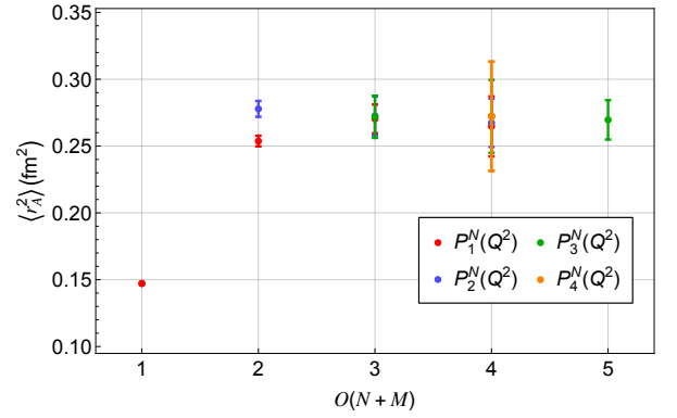
FIG. 6: Convergence pattern of the mean squared axial radius for the PA series P_1^N(Q^2) (red), P_2^N(Q^2) (blue), P_3^N(Q^2) (green) and P_4^N(Q^2) (orange) fitted to the Lattice QCD dataset.
