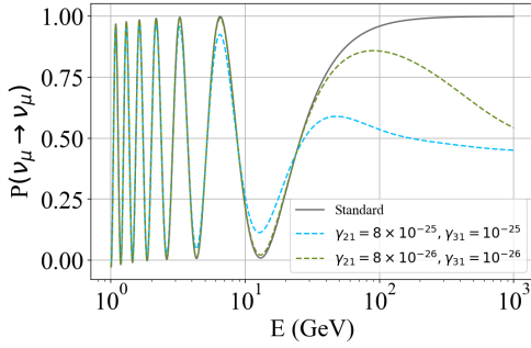
FIG. 1: Oscillation probability of a muon neutrino in vacuum. Solid line is standard oscillation, blue and green dashed line are deviations due to the decoherence parameters in the legend. The dependency on energy is n=1 .
