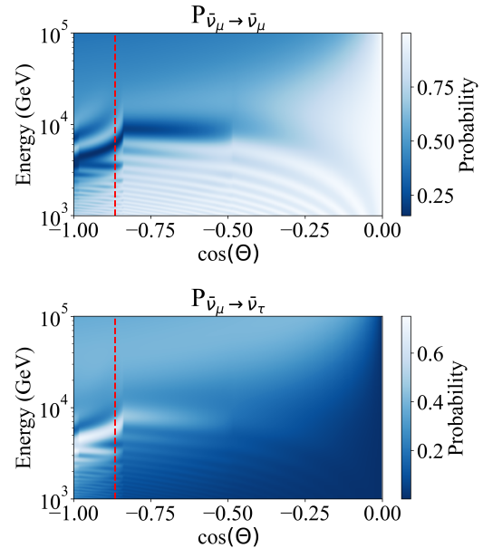
FIG. 5: Oscillograms for the muon antineutrino probabilities assuming normal mass ordering. Decoherence parameters are \gamma_{32} = \gamma_{31} = \gamma_{21} = 10^{-27} GeV, with an exponential dependency on energy of n=1 . The red line marks 150^\circ , constant angle represented at FIG. 7.
