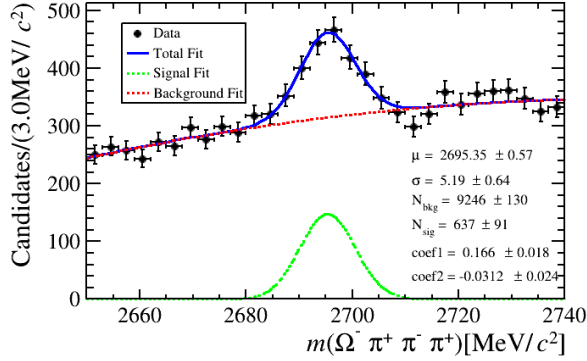
FIG. 4: Combined invariant mass distribution of \Omega_c^0 candidates from the DDL and DDD track categories, after applying all selection criteria.
