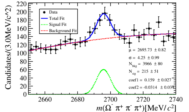
FIG. 3: Invariant mass distribution of \Omega_c^0 candidates in the DDD track category, after applying all selection criteria.
