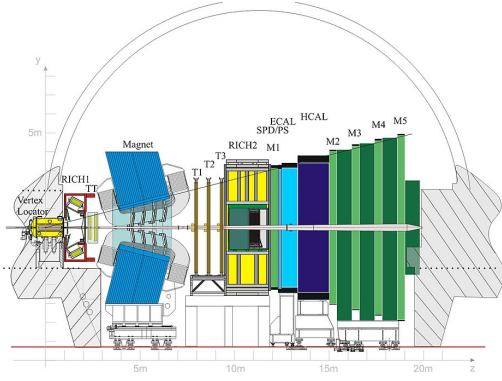
FIG. 1: Schematic side view of the LHCb detector, showing its main subdetectors.
