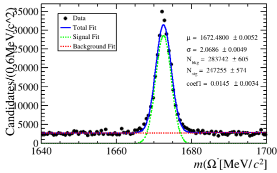
FIG. 8: Invariant mass distribution of \Omega^- candidates in the LLL category.
