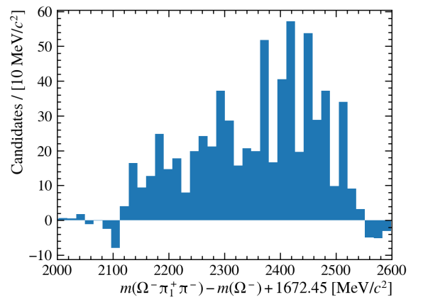
FIG. 6: Invariant mass spectrum of \Omega^- \pi^+ \pi^- using one pion pairing, weighted with the sWeightss . A mild enhancement is observed near 2470 MeV/c 2 .
