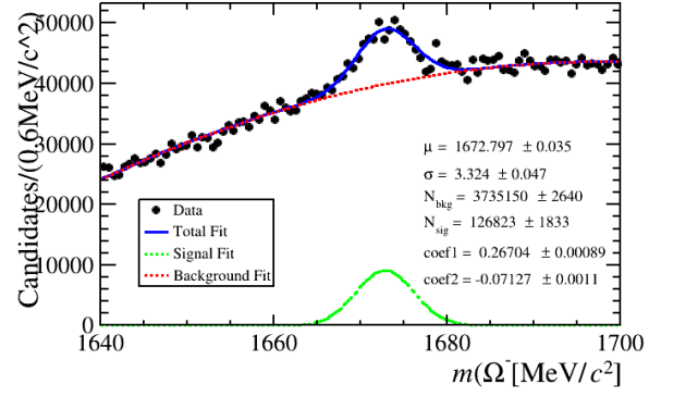
FIG. 10: Invariant mass distribution of \Omega^- candidates in the DDD category.
