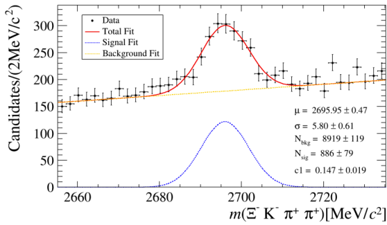
FIG. 5: Distribution of \Omega_c^0 invariant mass candidates in the DDL category from the decay \Omega_c^0 \rightarrow \Xi^- K^- \pi^+ \pi^+ , as obtained in [13]. Used for comparison with the current analysis based on the \Omega^- \pi^+ \pi^- \pi^+ channel.
