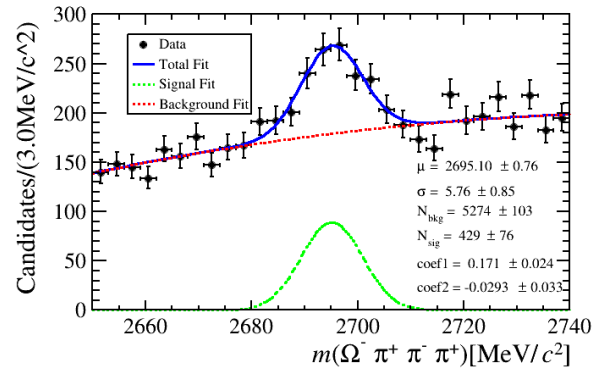
FIG. 2: Invariant mass distribution of \Omega_c^0 candidates in the DDL track category, after applying all selection criteria.
