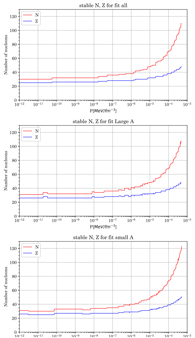
FIG. 7: Comparison of the nuclei that minimize de Gibbs energy for each data fit considered. The heavier the nuclei considered for the fitting of the parameters reach the drip line earlier, while fitting for lighter nuclei allows to have more neutron-richness in the atomic structure before reaching the drip line.
