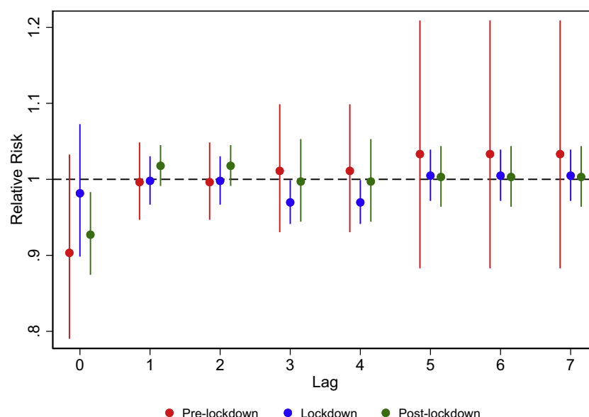
Fig. 4. Lagged effects of mean temperature (°C) on daily incidence of COVID-19 in Catalonia before, during, and after the lockdown periods.
