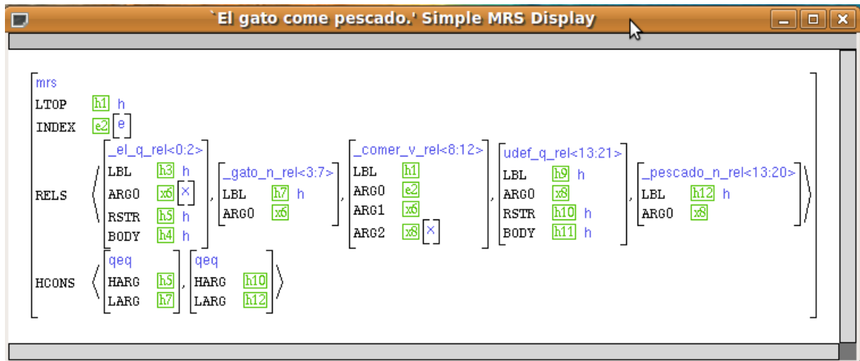
Figure 3: MRS semantic representation.
