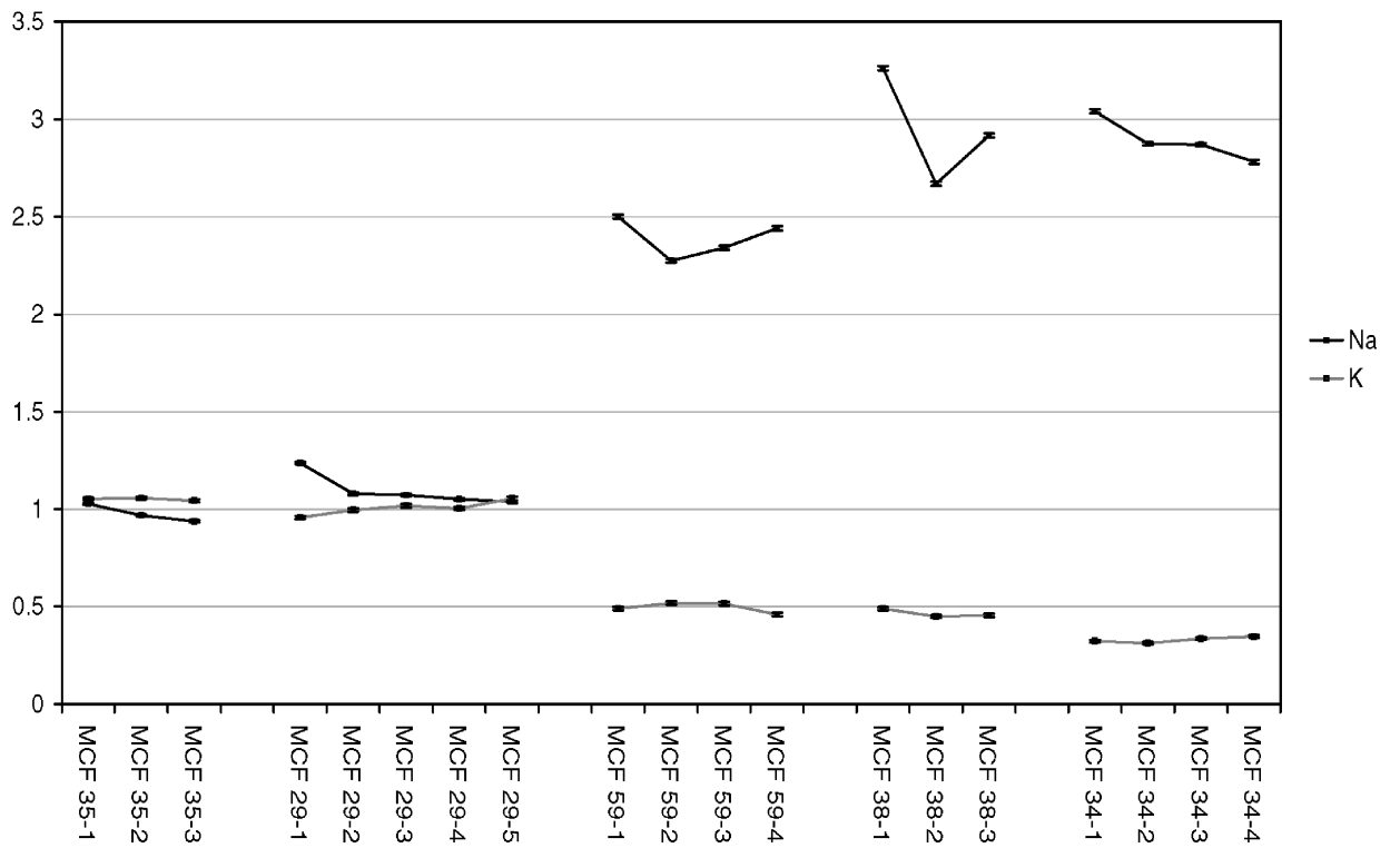
MCF alkali profiles normalized to core samples without analcime
