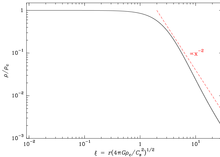
Figure 3.1: Numerical solution of the BE sphere density profile (Eq. 3.8) in logarithmic scale. \xi is the non-dimensional radius (Eq. 3.7) and \rho/\rho_c is the non-dimensional density.
