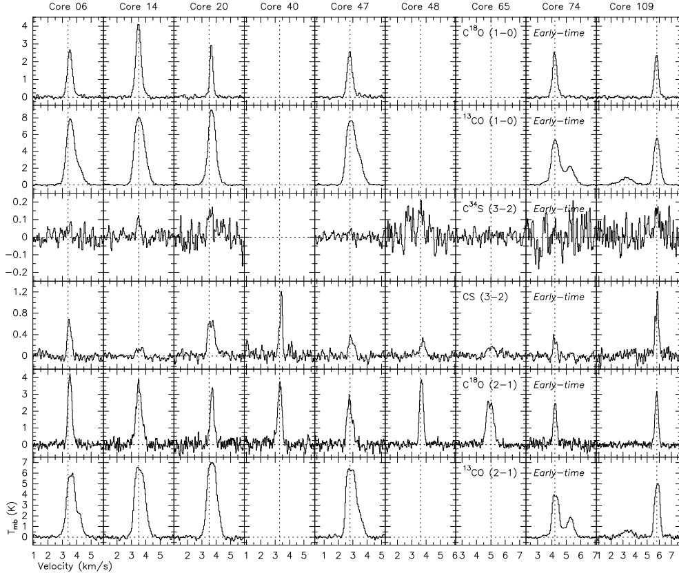
Figure 12. IRAM 30-m line spectra of the molecular transitions without hyperfine components toward the nine selected cores of the Pipe nebula (Table 1). These molecular transitions are not presented in Paper I. Columns: single cores named above the top panel of each column. Rows: single molecular transition specified on the seventh column. Empty panels represent non-observed molecular lines. Axes and dotted lines are as in Fig. 8. The velocity range is 5 \text{ km s}^{-1} except for Core 109 ( 6 \text{ km s}^{-1} ).
