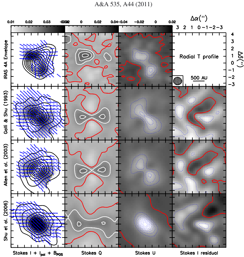
Fig. 8. Same as Fig. 7 for the case with the Maret et al. (2002) observational temperature gradient.
