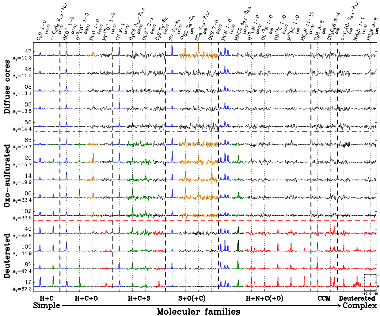
Fig. 2. Selected normalized molecular transitions toward the observed cores. The scale is shown in the bottom right spectrum. The normalized intensity axis ranges from -0.33 to 1 , while the velocity axis spans 20 \text{ km s}^{-1} centered at the v_{\text{LSR}} . Rows: individual cores, labeled on the left-hand side of the figure, ordered by its A_V peak. Columns: molecular transition, ordered by molecular families, labeled on the top of the figure. The spectra have been divided by [A_V/100 \text{ mag}] to mimic the abundance, where the A_V value is that at the respective core center (Román-Zúñiga et al. 2010) given below the core name. Each molecular transition has been multiplied by a factor, given below its name, to fit in a common scale. Colors are used to highlight the distinctive emission of the different core groups: blue for ubiquitous lines, green dense-medium molecular transitions, orange molecular transitions typical in oxo-sulfurated cores (see Sect. 4), red molecular transitions typical in deuterated cores, and black mostly undetected species.
