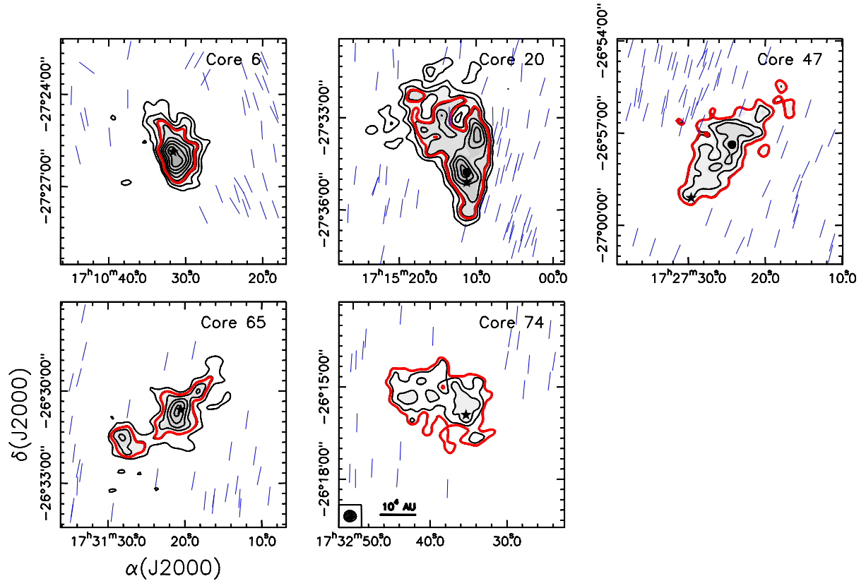
Figure 2. IRAM 30-m MAMBO-II maps of the dust continuum emission at 1.2 mm toward five cores of the Pipe nebula. The grayscale levels for all the maps are 3 to 18 times 5.75 \text{ mJy beam}^{-1} . The contour levels are 3 to 10 times \sigma in steps of 1-\sigma , where 1-\sigma is 4.0, 4.5, 4.9, 4.4, and 4.3 \text{ mJy beam}^{-1} for core 06, 20, 47, 65, and 74, respectively. The red thick contour marks the half maximum emission level of the source (Table 3). Black stars indicate the \text{C}^{18}\text{O} pointing center reported by Muench et al. (2007). Black filled circles indicate the position where line observations have been performed, if different from the Muench et al. (2007) position, closer to the dust continuum emission maximum which falls into the beam area. The blue vectors depict the polarization vectors found by Franco et al. (2010). In the bottom left corner of the bottom middle panel the convolved beam and the spatial scale for the maps are shown.
