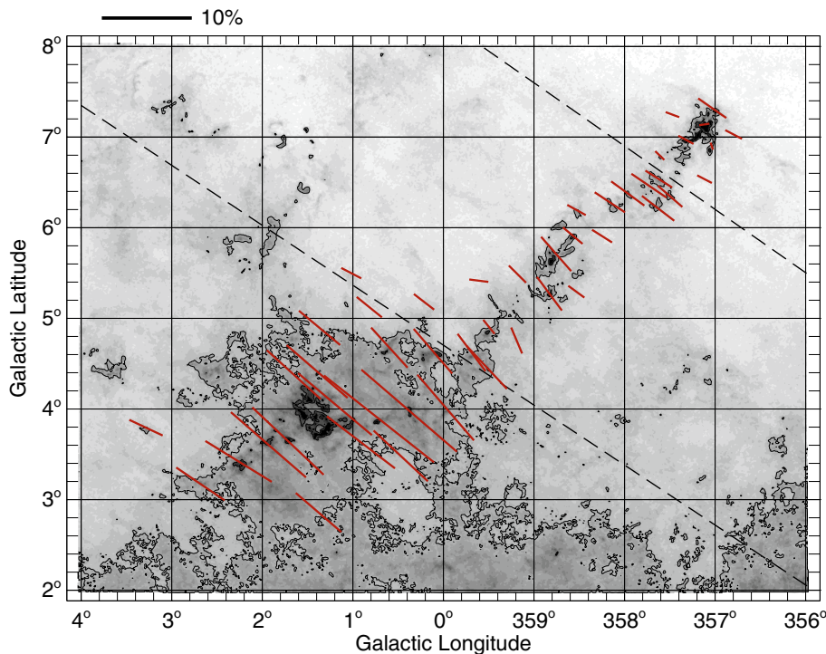
Figure 4.1: Mean polarization vectors of the fields observed with optical polarimetry toward the Pipe nebula extracted from Alves et al. (2008). The lengths of the vectors are proportional to the degree of polarization indicated in the top left-hand corner. The A_V map is that of Lombardi et al. (2006). The overall magnetic field is perpendicular to the filamentary structure.
