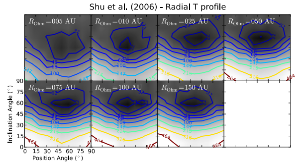
Fig. 10. Same as Fig. 3 for the Shu et al. (2006) model with radial temperature profile.
