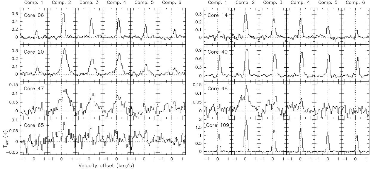
Figure 11. IRAM 30-m line spectra of C_2H (1–0) ( early-time ) toward eight cores of the Pipe nebula (Table 1). This molecular transition is not presented in Paper I. The component number following Padovani et al. (2009) is indicated above each column. The name of the core is indicated in the left panel of each row. Axes and dotted lines are as in Fig. 8. The velocity range is 2.5 \text{ km s}^{-1} .
