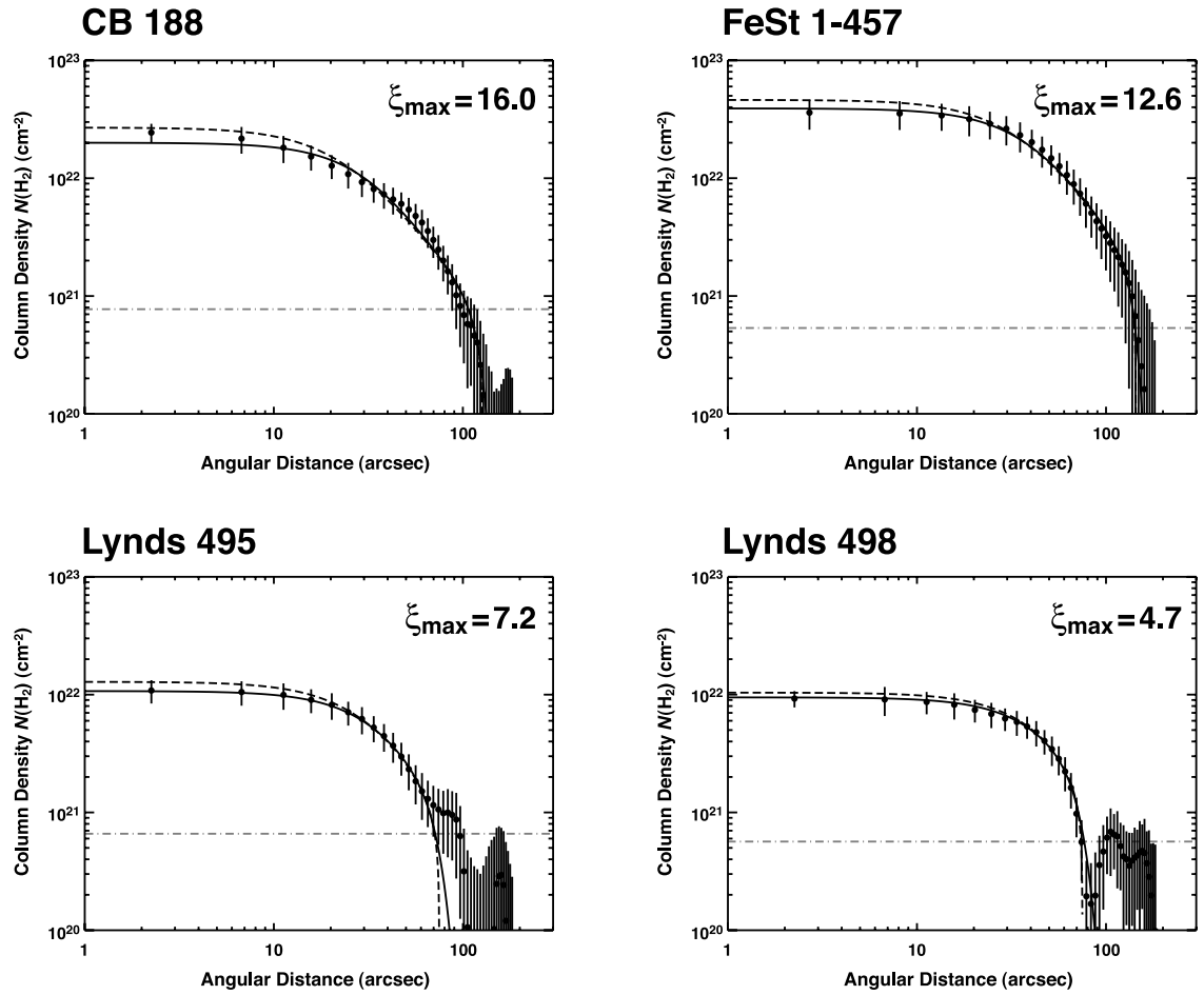
Figure 3.4: Radial column density profiles of four Bok globules extracted from Kandori et al. (2005). Circles and bars show the average and rms dispersion for each radial annulus. The solid line represents the best fit of a theoretical BE sphere to the data. The values of \xi_{\max} indicate that three of the four are thermally unstable to gravitational collapse.
