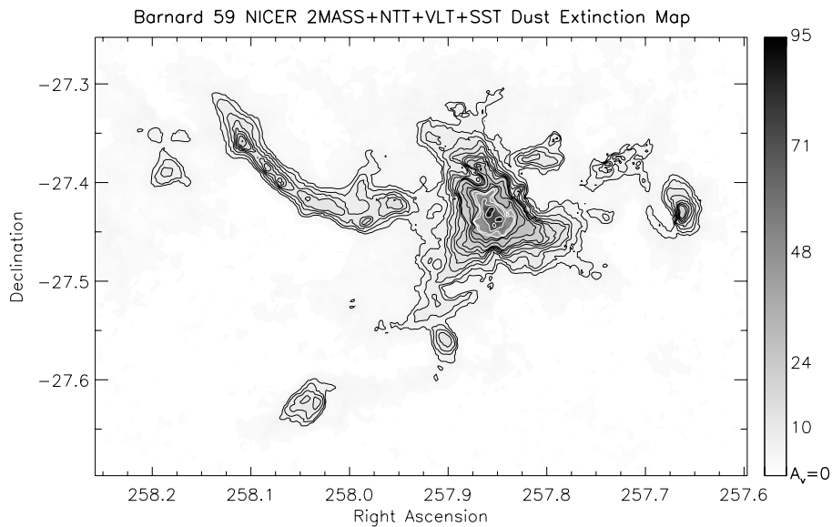
Figure 4.2: Extinction map of Barnard 59 at a resolution of \sim 20'' extracted from Román-Zúñiga et al. (2009). The black solid line contours mark levels of extinction from A_V=6.0 to 20.0 mag in 2.0 mag increments, and from A_V=20.0 to 35.0 mag in 5.0 mag increments; the white contours mark levels of extinction at 40, 45, 60, and 80 mag.
