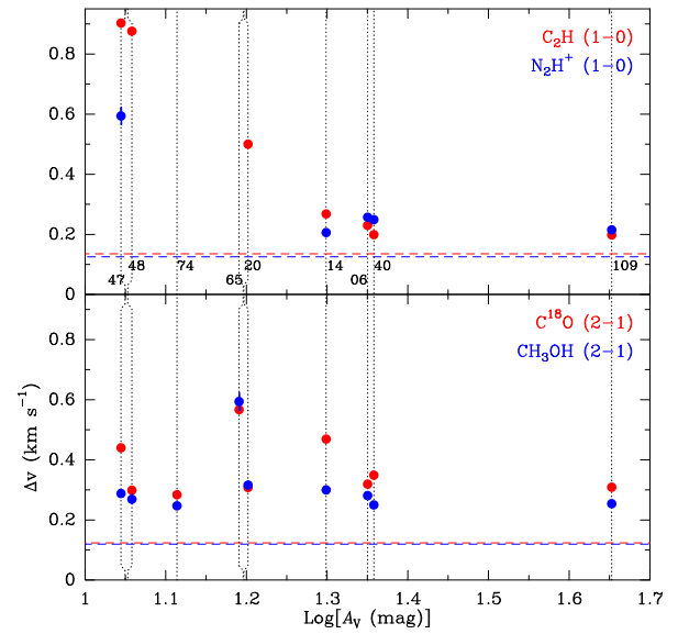
Figure 7. Top panel : line width of the \text{C}_2\text{H} (1–0) and \text{N}_2\text{H}^+ (1–0) lines, colored in red and blue, respectively, as a function of the logarithm of the core A_V peak. Bottom panel : Same as top panel but for the \text{C}^{18}\text{O} (2–1) and \text{CH}_3\text{OH} (2–1) lines, colored in red and blue, respectively. Colored dashed horizontal lines show the corresponding thermal line width for each molecule for a temperature of 10 K. Vertical dotted lines mark the A_V peak of each core, which in the case of similar values (cores 47 and 48, and 20 and 65) have been slightly displaced.
