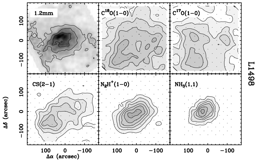
Figure 3.14: Selective molecular freeze-out toward L1498 extracted from Tafalla et al. (2002). Carbon-bearing molecules deplete at high densities and show a ring-like structure. On the other hand, nitrogen-bearing molecules trace the core center in good agreement with the continuum dust emission map.
