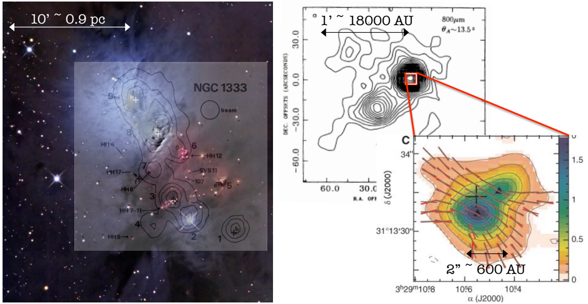
Figure 4.3: Left : Optical image of the reflection nebula NGC 1333 (APOD; April 18, 2009) with several contours of the 50\mu\text{m} map overlaid (Jennings et al., 1987). IRAS 4 is located in the bottom middle part. Top right : Contours of the submillimeter continuum emission of NGC 1333 IRAS 4 (Sandell et al., 1991), IRAS 4A is the source located at the N-E end of the cloud. Bottom right : close up view of IRAS 4A in submillimeter continuum emission (Girart et al., 2006). Red bars show the measured magnetic field vectors. Gray bars show the best-fit parabolic magnetic field model. The pinched magnetic field displays a clear “hourglass” morphology.
