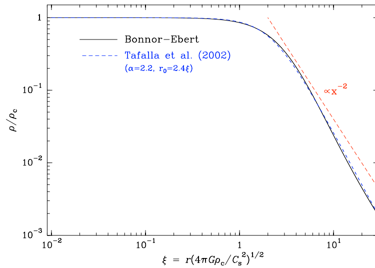
Figure 3.7: Same as Fig. 3.1. The blue dashed line depicts the density profile from Eq. 3.52 using r_0 = 2.4\xi and \alpha = 2.2 . The agreement to the BE profile is remarkable.
