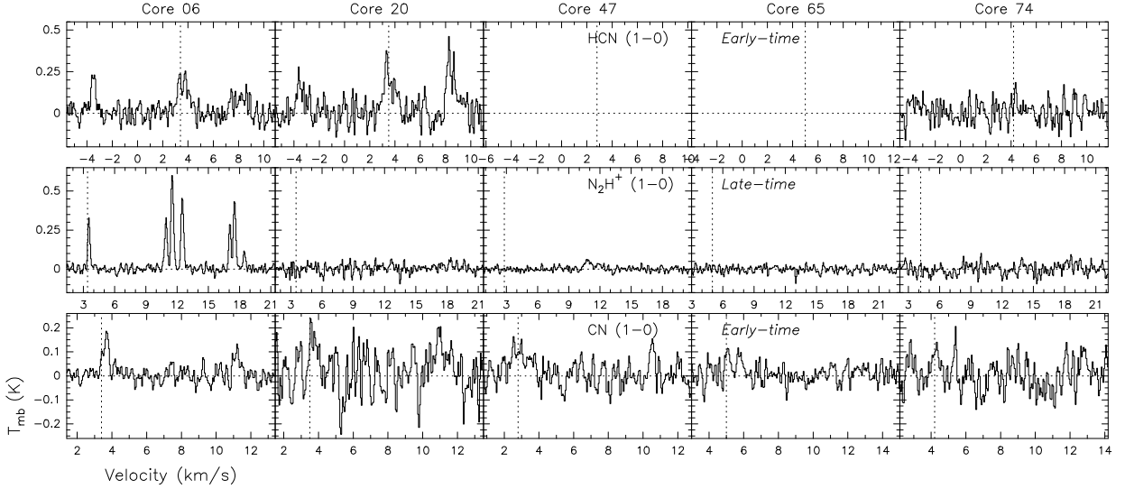
Figure 8. IRAM 30-m line spectra of the molecular transitions with hyperfine components presented in Paper I toward the five new selected cores of the Pipe nebula presented in this work (Table 1). Columns: single cores named above the top panel of each column. Rows: single molecular transition specified on the third column. Empty panels represent non-observed molecular lines. The velocity range is 16.5, 20 and 12 km s -1 for HCN (1–0), N 2 H + (1–0), and CN (1–0), respectively. Horizontal axis shows the velocity, and the v LSR of each core is marked with a vertical dotted line. Vertical axis shows the T MB of the emission, and the zero level is marked by a horizontal dotted line.
