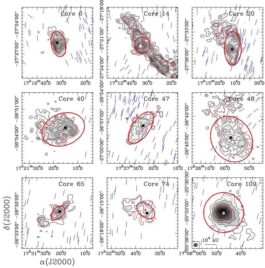
Fig. 1. IRAM 30-m MAMBO-II maps of the dust continuum emission at 1.2 mm toward nine cores of the Pipe nebula presented in Papers I and II. In the bottom left corner of the bottom right panel the convolved beam and the spatial scale for the maps are shown. Grayscale : levels are common for all the maps and range from 3 to 18 times 5.75 \text{ mJy beam}^{-1} . Contour levels : 3 to 10 times \sigma in steps of 1\text{-}\sigma for all the cores but core 109, for which the contour levels are 3 to 21\sigma in steps of 3\sigma . 1\text{-}\sigma is 4.0, 4.5, 4.5, 5.0, 4.9, 3.5, 4.4, and 4.3 \text{ mJy beam}^{-1} for cores 06, 14, 20, 40, 47, 48, 65, 74, and 109, respectively. Red thin contour : half maximum emission level of the source (see Table 1). Black or white filled circles : line observation pointing positions of Paper I and Paper II, very close to the dust continuum emission maximum. Blue vectors : polarization vectors found by Franco et al. (2010). Red cross : center of the concentric rings used to calculate the intensity profile. Red thick ellipse : external boundary of the best fitting Bonnor-Ebert profile.
