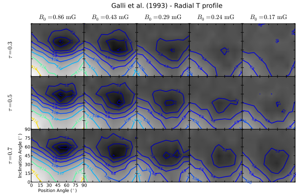
Fig. 3. Pixel map: sum of the \chi^2 of the Stokes Q and U maps for the Galli & Shu (1993a,b) model with radial temperature profile with respect to the data. Contours: 10, 10^{1/6} , 10^{2/6} , ..., 10^3 \chi^2 levels.
