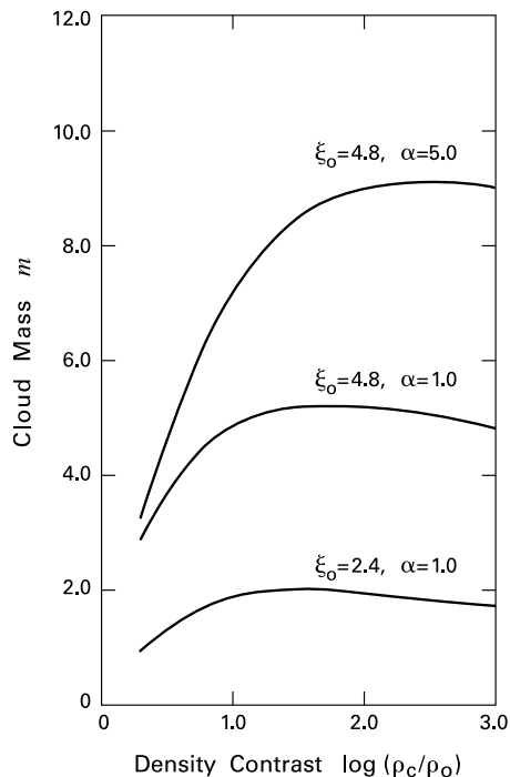
Figure 3.6: Non-dimensional critical mass, m_{\text{crit}} , in equilibrium configurations of magnetized clouds (based on Tomisaka et al., 1988b, extracted from Stahler & Palla, 2005). m_{\text{crit}} is plotted as a function of the density contrast for selected combinations of \xi_0 and \alpha .
