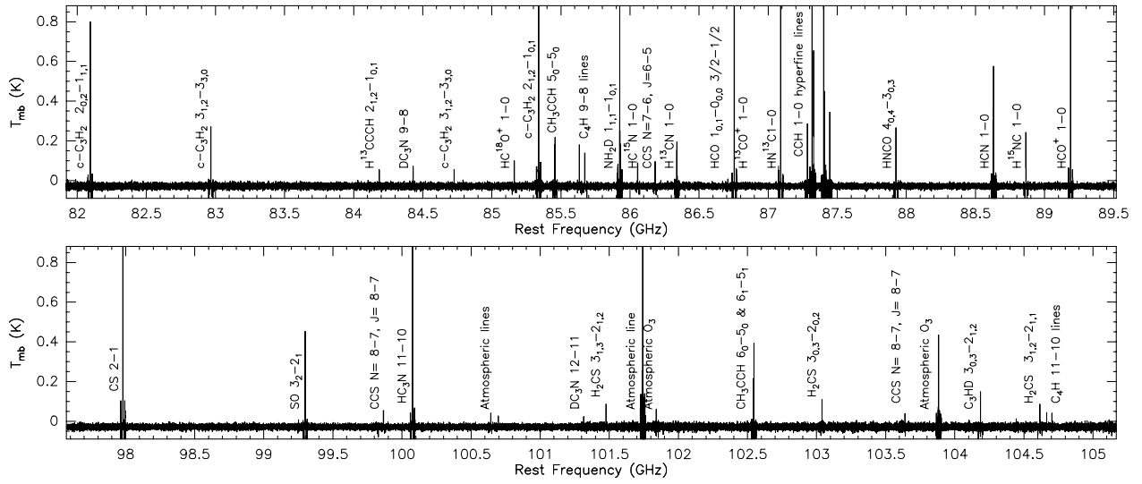
Fig. 1. IRAM 30-m EMIR+FTS full bandwidth spectrum toward core 12. The most important detected molecular transitions are labeled within the plot. The upper and lower panels show the \sim 7.6 GHz lower and upper sidebands, respectively. The noise rarely exceeds 10 mK. The negative emission are the twin negative counterparts of the positive emission due to the frequency-switching observing mode.
