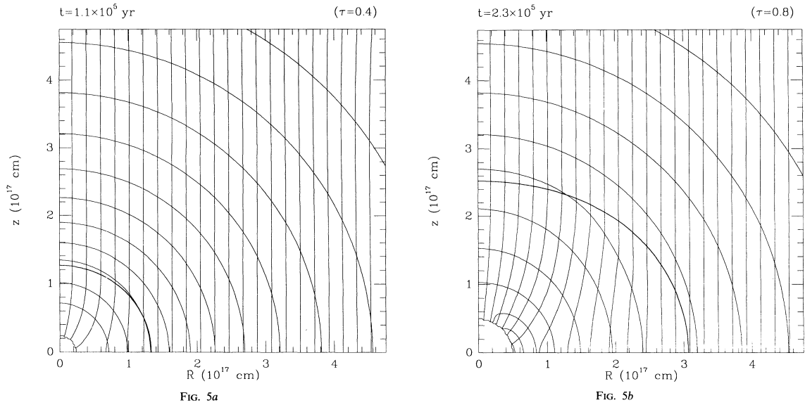
Figure 3.11: Semi-analytical solution for the time evolution of an infalling spherical dense core with ambipolar diffusion extracted from Galli & Shu (1993a). Density contours and magnetic field lines are shown. The infall wave front is depicted as a black thick contour. The semi-analytical solution fails toward the inner part and has been clipped.
