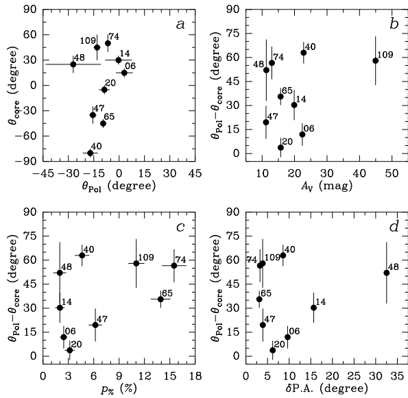
Figure 6. Relation of the core major axis orientation ( \theta_{\text{core}} ) to different physical parameters. a : \theta_{\text{core}} against mean polarization angle ( \theta_{\text{pol}} ) of the corresponding observed field (Franco et al. 2010). b-d : \theta_{\text{pol}} - \theta_{\text{core}} as a function of core A_V peak (Román-Zúñiga et al. 2009, 2010), polarization fraction ( p\% ) and polarization angle dispersion ( \delta\text{P.A.} ), respectively.
