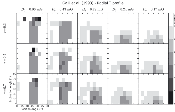
Fig. 2. Pixel map: standard deviation of the difference of the synthetic polarization vectors with respect to the observed ones for the Galli & Shu (1993a,b) model with radial temperature profile. White pixels represent excluded models (see text). Grayscale is on the right-hand side of the figure.
