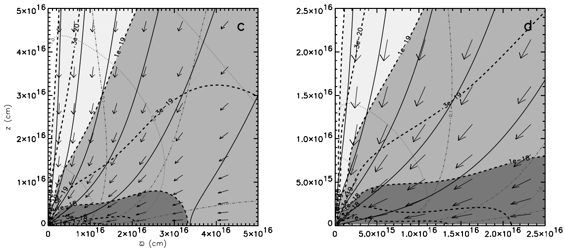
Figure 3.12: Snapshot of the inner region of a numerical simulation of an infalling magnetized toroid with ambipolar diffusion extracted from Allen et al. (2003a). Density contours (dashed lines), magnetic field lines (solid lines), and local velocities (arrows) are shown. The flow deflection due to magnetic fields forms a pseudo-disk around the protostar.
