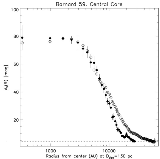
Figure 2. Open circle symbols show the radial profile of the NICER extinction map. The black diamond symbols show the radial profile of the MAMBO-II dust emission map. The profiles were constructed by averaging flux in circular, concentric rings centered on J2000 (\alpha, \delta) = (17:11:23.0, -27:25:59.3) . For the MAMBO-II profile, the data were convolved to the resolution of the NICER map ( 20'' ) and re-gridded to match pixels in both maps.
