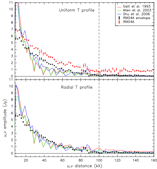
Fig. 6. Stokes I visibility amplitudes vs. u, v distance averaged in bins of 2k\lambda . Top panel: uniform temperature profile. Bottom panel: radial temperature profile. Red and black dots: IRAS 4A full data and envelope data, respectively, with their statistical error bars. Vertical dashed line: u, v distance threshold used to derive the compact components map (see Fig. 1). Starting at \sim 90 k\lambda the emission seems to match with an unresolved source of \sim 1 Jy. Red, green, and blue solid curves: visibility amplitudes derived after convolving the Galli & Shu (1993a,b), Allen et al. (2003a,b), and Shu et al. (2006) models, respectively, used to generate the maps of left-hand panels of Figs. 7 and 8.
