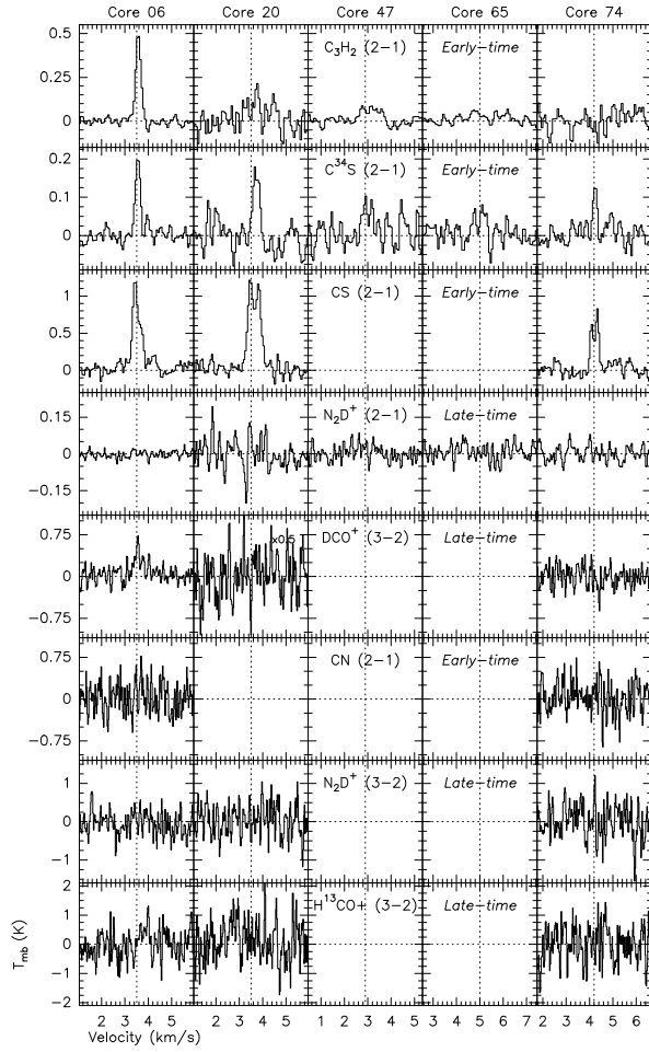
Figure 9. IRAM 30-m line spectra of the molecular transitions without hyperfine components presented in Paper I toward the five new selected cores of the Pipe nebula presented in this work (Table 1). Columns: single cores nebula presented in this work (Table 1). Rows: single molecular transition specified on the third column. Empty panels represent non-observed molecular lines. Axes and dotted lines are as in Fig. 8. The velocity range is 5 \text{ km s}^{-1} centered on the v_{\text{LSR}} of each core.
