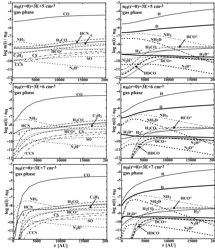
Figure 3.15: Gas-phase chemistry in a contracting BE sphere extracted from Aikawa et al. (2005). Radial distribution of the calculated abundances at n(\text{H}_2) = 3 \times 10^5 \text{ cm}^{-3} (top panels), 3 \times 10^6 \text{ cm}^{-3} (middle panels), and 3 \times 10^7 \text{ cm}^{-3} (bottom panels).
