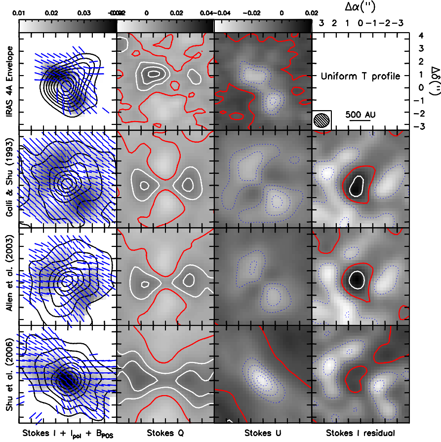
Fig. 7. Comparison of selected models with data assuming a uniform temperature of the gas. The orientation angles are fixed to \phi = 50^\circ and \omega = 45^\circ for a better model comparison. Rows: IRAS 4A (first row); model Galli & Shu (1993a,b) with B_0 = 0.43 and \tau = 0.7 (second row); model Allen et al. (2003a,b) with H_0 = 0.125 , v_0 = 0 and t = 10^4 yr (third row); and model Shu et al. (2006) with r_{\text{ohm}} = 75 AU (fourth row). Columns: in each row, the panels show: intensity (first panel, contours), polarized intensity (first panel, pixel map) and magnetic field vectors (first panel, segments); map of Stokes Q (second panel, pixel map and contours); map of Stokes U (third panel, pixel map and contours); residuals models-data for Stokes I (fourth panel, pixel map and contours). The color scale is shown on the top of each column. Contours: contours for the Stokes I maps (left panels) depict emission levels from 6\sigma up to the maximum value in steps of 6\sigma , where \sigma = 0.02 Jy beam ^{-1} . Contours for the Stokes Q and U maps depict levels from the minimum up to the maximum in steps of 3\sigma where \sigma = 2.5 mJy beam ^{-1} . The solid red contour marks the zero emission level, solid white contours mark positive emission and blue dotted contours mark negative emission. Contours for the residual Stokes I follow the same rule of Stokes Q and U but with steps of 6\sigma , where \sigma = 0.02 Jy beam ^{-1} . The top right panel shows the beam and the angular and spatial scale.
