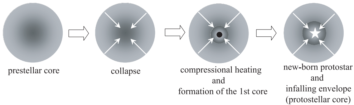
Figure 3.13: Evolution of a star-forming core extracted from Aikawa et al. (2008)
