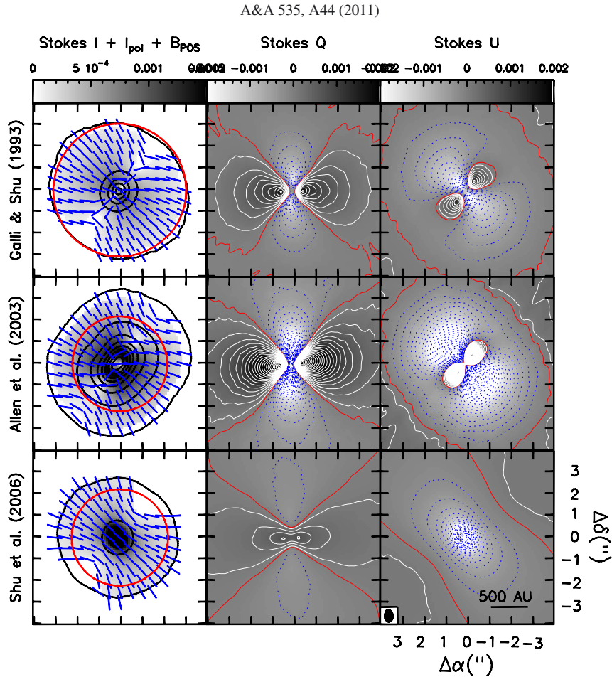
Fig. 11. Same as Fig. 8 for ALMA configuration 09. Contours: contours for the Stokes I maps (left panels) depict emission levels from 5\sigma up to the maximum value in steps of 50\sigma , where \sigma = 0.2 \text{ mJy beam}^{-1} . Positive contours for the Stokes Q and U maps depict levels from 5\sigma up to the maximum in steps of 10\sigma , where \sigma = 0.02 \text{ mJy beam}^{-1} . Negative contours follow the same rule. Red circles: for the Galli & Shu (1993a,b) and Allen et al. (2003a,b) models depict the loci of the front of the isothermal collapse wave ( r = c_s t , see Fig. 2 of Galli & Shu 1993a and Fig. 6 of Allen et al. 2003a). For the Shu et al. (2006) model it marks the 10 r_{\text{Ohm}} distance (see Fig. 4 of Shu et al. 2006).
