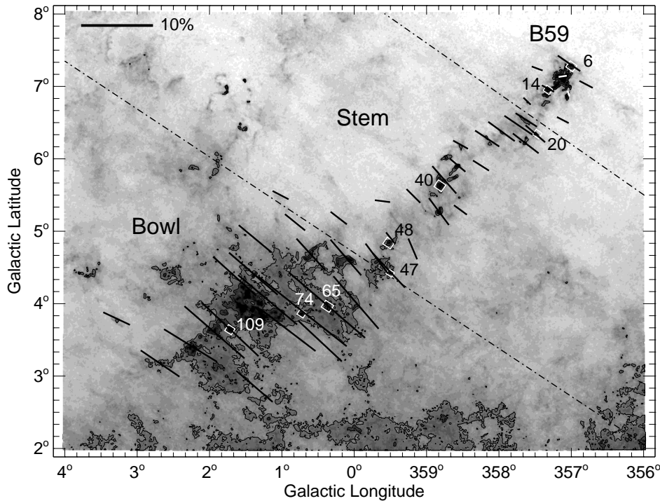
Figure 1. Position of the observed cores plotted over the 2MASS extinction map of the Pipe nebula (Lombardi et al. 2006). Black segments represent the mean polarization vector of the region (Alves et al. 2008) with the scale shown on the top left corner of the figure. White boxes depict the size of the 1.2 mm continuum maps (Section 2.1 and Fig. 2 of both Paper I and the present work). The dashed lines separate the three different magnetically defined regions (Alves et al. 2008). The lowest visual extinction ( A_V ) corresponds to 0.5 magnitudes. The highest A_V is observed toward the bowl and B59 regions, where it reaches approximately 20 magnitudes.
