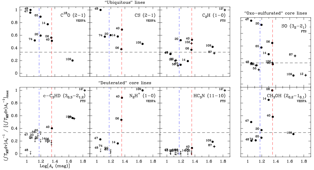
Figure 4. Normalized integrated intensity ( A_V^{-1} \int T_{MB} dv ) of selected molecular transitions divided by its maximum value as a function of the logarithm of the core A_V peak. Each panel shows the molecular transition in the top right corner. The backend is labeled below the molecular transition: VESPA panels present the nine cores of Paper I and present work, while FTS panels present the fourteen cores of Paper II. Filled circles represent the nine cores of Paper I and present work, stars represent the other six cores from Paper II (08, 12, 33, 56, 87, and 102), and arrows represent upper limits. Molecules have been split into the three categories defined in Paper II, labeled on the top of each group. The blue dot-dashed and red dashed vertical lines mark the transition from “diffuse” to “oxo-sulfurated”, and from “oxo-sulfurated” to “deuterated” cores, respectively. The horizontal dashed line marks a third of the peak value which helps to show the behavior change of the “oxo-sulfurated” and “deuterated” lines in our sample. The maximum values for each molecular transition are, in \text{K km s}^{-1} \text{mag}^{-1} , 0.114, 0.036, and 0.030 for the ubiquitous \text{C}^{18}\text{O} , CS, and \text{C}_2\text{H} , 0.059 and 0.025 for the “oxo-sulfurated” SO and \text{CH}_3\text{OH} , and 0.003, 0.010, and 0.019 for the “deuterated” c\text{-C}_3\text{HD} , \text{N}_2\text{H}^+ , and \text{HC}_3\text{N} , respectively.
