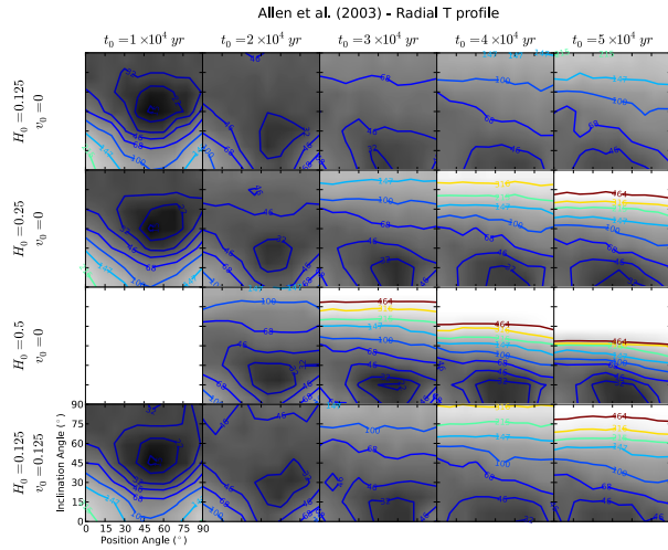
Fig. 9. Same as Fig. 3 for the Allen et al. (2003a,b) model with radial temperature profile.
