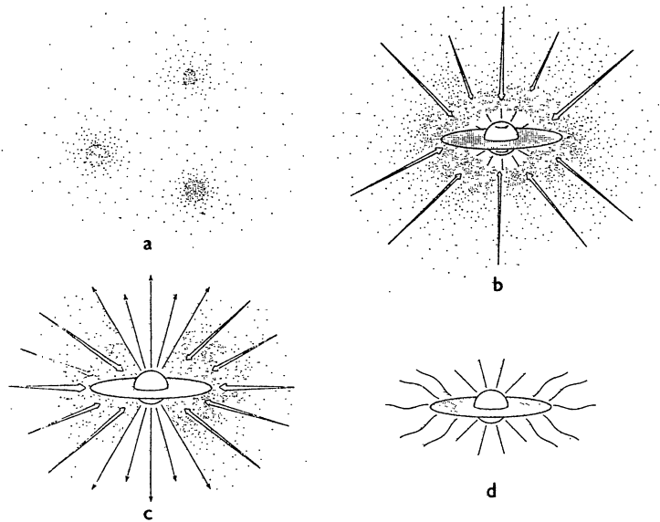
Figure 2.1: The four stages of low-mass star formation extracted from Shu et al. (1987) (a) Cores form within molecular clouds as magnetic and turbulent support is lost through ambipolar diffusion. (b) A protostar with a surrounding nebular disk forms at the center of a cloud core collapsing inside-out. (c) A stellar wind breaks out along the rotational axis of the system, creating a bipolar flow. (d) The infall terminates, revealing a newly formed star with a circumstellar disk
