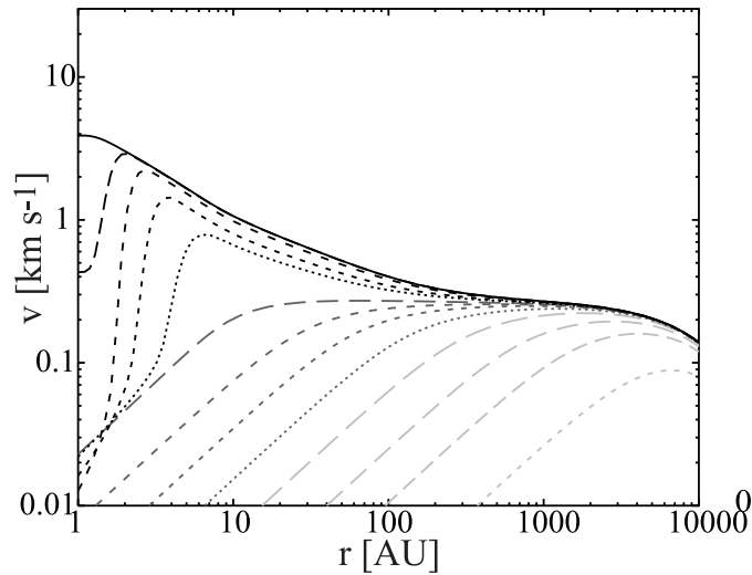
Figure 3.8: Radial distribution of velocity in a collapsing BE extracted from Aikawa et al. (2008). Their calculations allow for temperature variations but the process remain essentially isothermal for a few 10^5 yr up to densities of n \sim 10^6 \text{ cm}^{-3} (dark gray dashed line). Times in yr. measured to the formation of the protostar for the "isothermal" profiles are, from right to left, -2.5 \times 10^5 , -1.1 \times 10^5 , -3.3 \times 10^4 , -1.5 \times 10^4 , -6.4 \times 10^3 , -3.4 \times 10^3 , -2.1 \times 10^3 , and -1.2 \times 10^3 .
