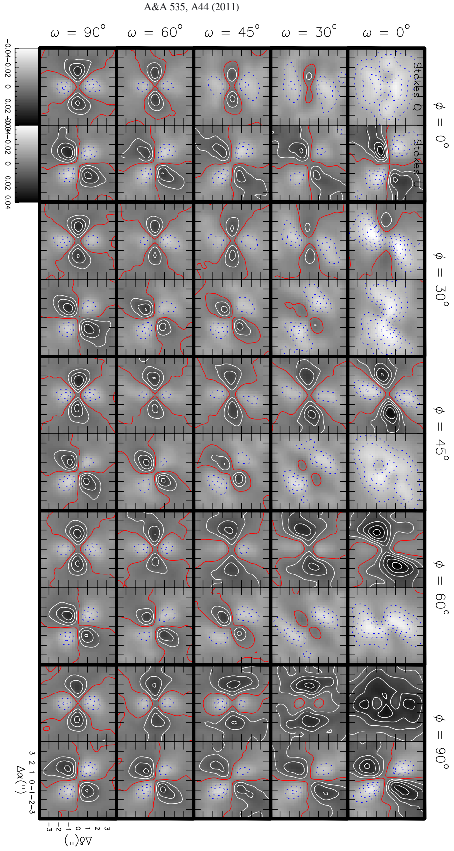
Fig. 4. Dependence of the synthetic Stokes Q and U maps on the orientation angles. The maps shown corresponds to the Allen et al. (2003a,b) model with H_0 = 0.125 , v_0 = 0 and t = 2 \times 10^4 yr. Thick contours: correspond to a single combination of position and inclination angle. Individual panels: inside thick contours two panels are shown. Stokes Q and U map are shown in the left- and right-hand side panels, respectively. Common color scale for each Stokes map is shown below the first column. The angular scale is shown in the bottom right-hand side panel. Map contours: represent steps of 3\text{-}\sigma starting at 3\text{-}\sigma , where \sigma = 2.5 mJy beam ^{-1} . Columns: correspond to a position angle, \phi , shown on the top. Rows: correspond to an inclination angle, \omega , shown on the left-hand side of the figure.
