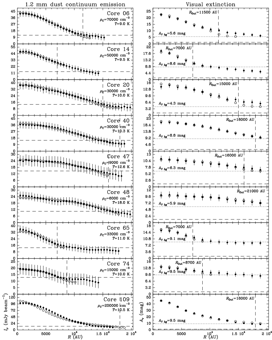
Fig. 2. Radial intensity profiles of the Pipe nebula starless cores presented in Papers I and II. Left column: intensity profile from the 1.2 mm dust continuum emission maps (Papers I and II). Right column: A_V profile from the dust extinction maps (Román-Zúñiga et al., 2009, 2010). Rows: each row corresponds to a single core labeled on left panels. Black dots: represent the observed values with vertical bars depicting the \pm 1\text{-}\sigma range. Empty circles: represent the value of the fitted Bonnor-Ebert profile. On each left panel, the best fitting central density, \rho_c , and dust temperature, T , are shown. The core boundary radius, R_{\text{out}} , and A_V value of the surrounding medium, A_V^{\text{bg}} , are labeled on right panels and shown as a vertical dashed line and horizontal dotted line, respectively. Horizontal dashed line represent the 3\text{-}\sigma level (left panels) or the cutoff A_V (right panels).
