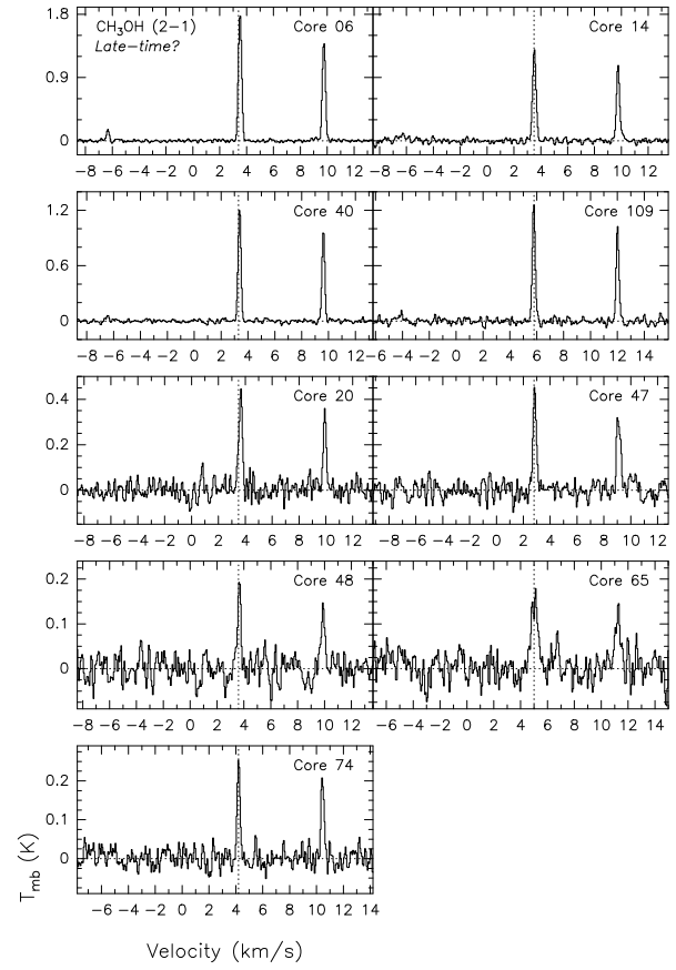
Figure 10. IRAM 30-m line spectra of \text{CH}_3\text{OH} (2-1) toward the nine selected cores of the Pipe nebula (Table 1). This molecular transition is not presented in Paper I. The name of the core is indicated in the top right corner of each panel. Axes and dotted lines are as in Fig. 8. The velocity range is 22 \text{ km s}^{-1} .
