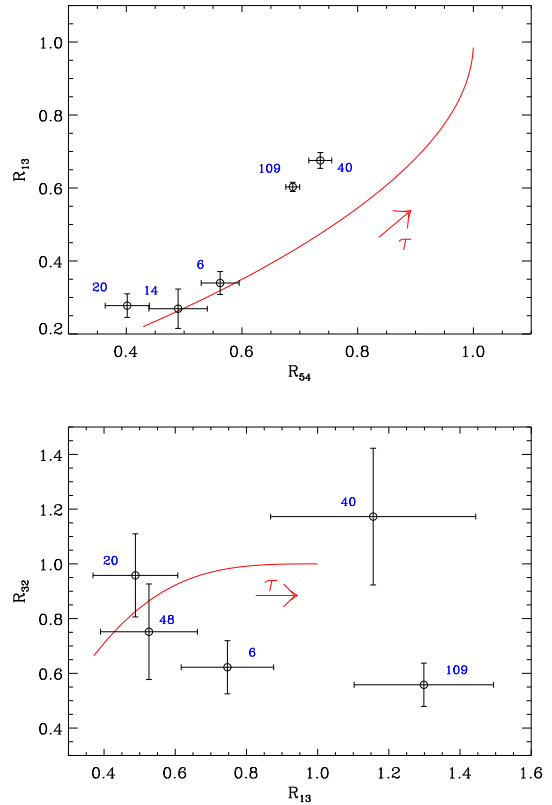
Figure 5. Ratio of the integrated intensities of couples of components of \text{C}_2\text{H} (1-0) (upper panel, see Table 5 in Padovani et al. 2009 for labels) and \text{HCN} (1-0) (lower panel, see Table B.1 in Padovani et al. 2011 for labels). Empty circles: observational data labeled with the respective core number. Red solid line: one-slab LTE model, optical depth increases in the arrow direction (see Padovani et al. 2009 for details).
