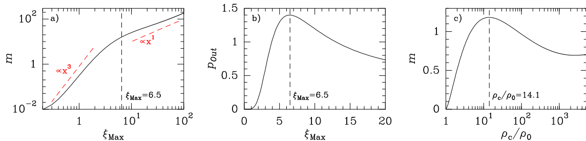
Figure 3.3: Numerical solution of the BE sphere. Left panel: non-dimensional mass m up to \xi = \xi_{\text{max}} as a function of \xi_{\text{max}} . Middle panel: Outer confining pressure as a function of \xi_{\text{max}} . Right panel: m up to \xi = \xi_{\text{max}} as a function of the density contrast.
