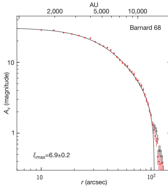
Figure 3.2: Radial column density profile of B68 extracted from Alves et al. (2001) in terms of magnitudes of A_V . Circles and bars show the data points and rms dispersion for the averaged profile of the extinction measurements. The solid line represents the best fit of a theoretical BE sphere to the data. The close match of the data with theory indicates that the internal structure of the cloud is well characterized by the equations for a self-gravitating, pressure-confined, isothermal sphere with gravity balanced by thermal pressure.
