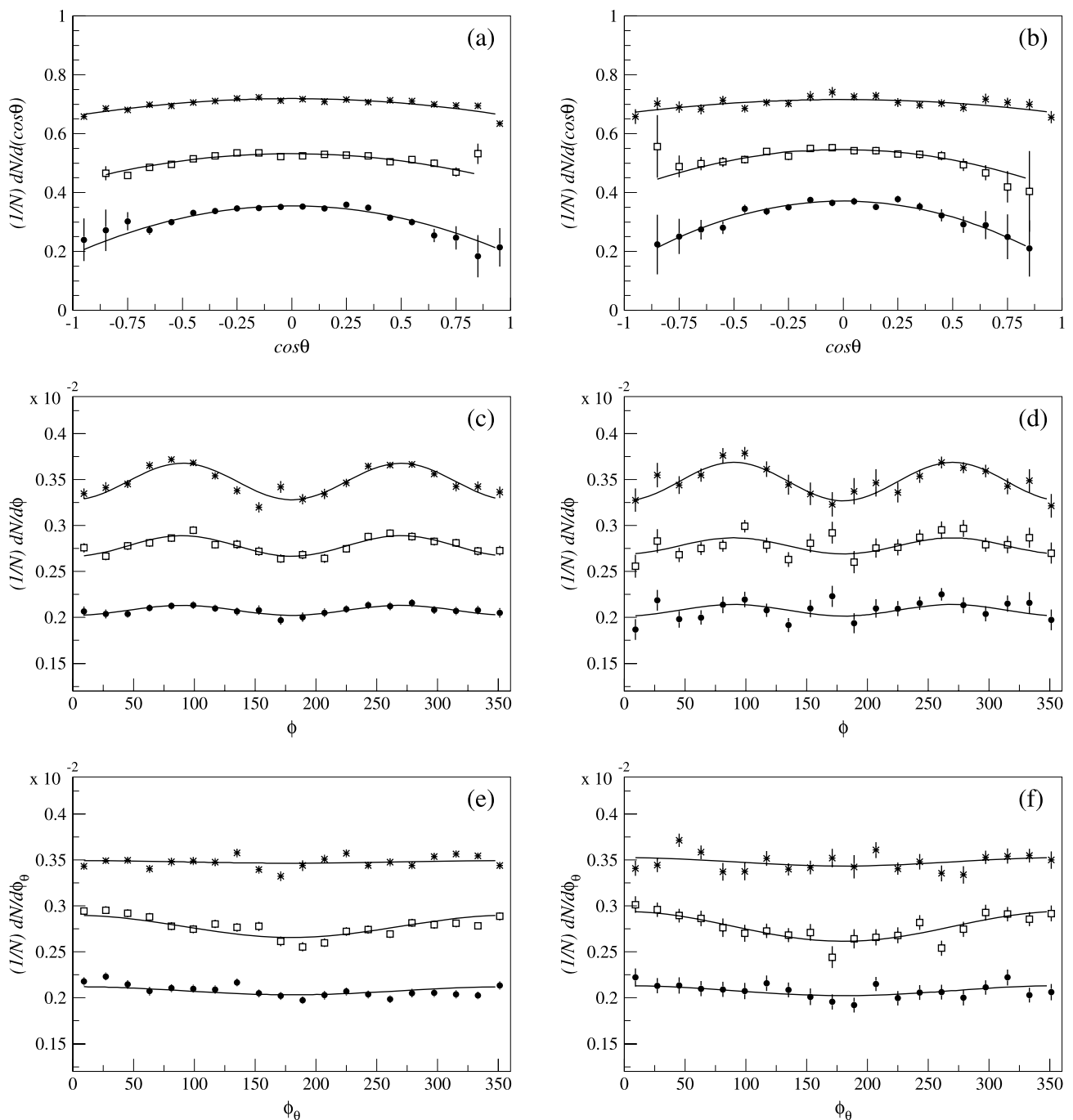
Fig. 3.1 Efficiency-corrected distributions of the angular variables \cos\theta (a, b), \phi (c, d) and \phi_\theta (e, f) measured in the muon (left column) and electron (right column) decay channels of the J/\psi over the whole visible phase space. The results obtained in the Collins-Soper, Gottfried-Jackson and helicity frames are represented, respectively, by
