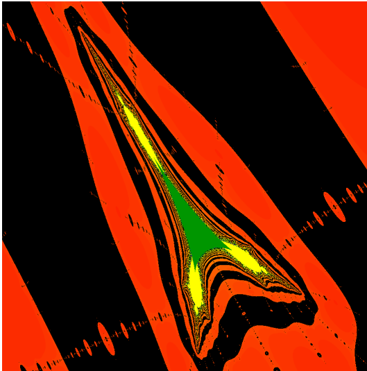
(c) A Tricorn-like set.
