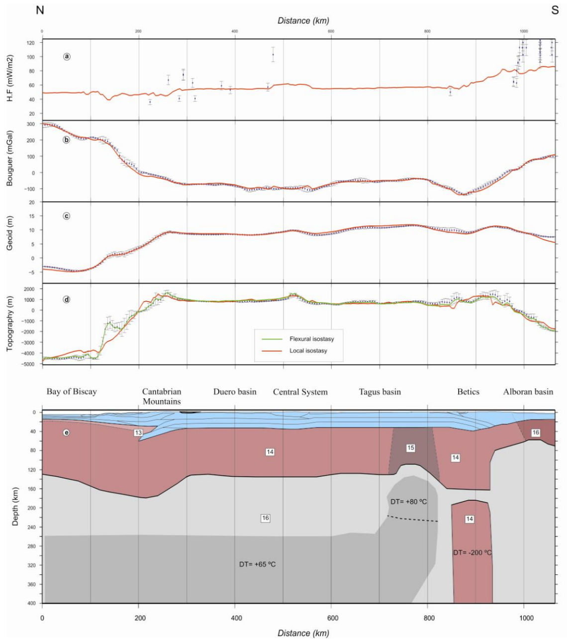
Figure 4.4: Model results (red lines), measured data with the standard deviation of data projected onto the profile within a strip of 25 km half-width (blue dots and vertical bars), coupled calculated topography (red line), and green line represent calculated elevation in the case of effective elastic thickness for the different T_e (30 km, 20 and 10 km) used along the profile (see text for details): (a) surface heat flow; (b) Bouguer anomaly; (c) geoid height; (d) elevation; (e) lithospheric structure. Crustal structure like in Figure 4.2. Numbers in panel (e) denote mantle bodies summarized in Table 4.1. Dataset sources as in Figure 1.3.
