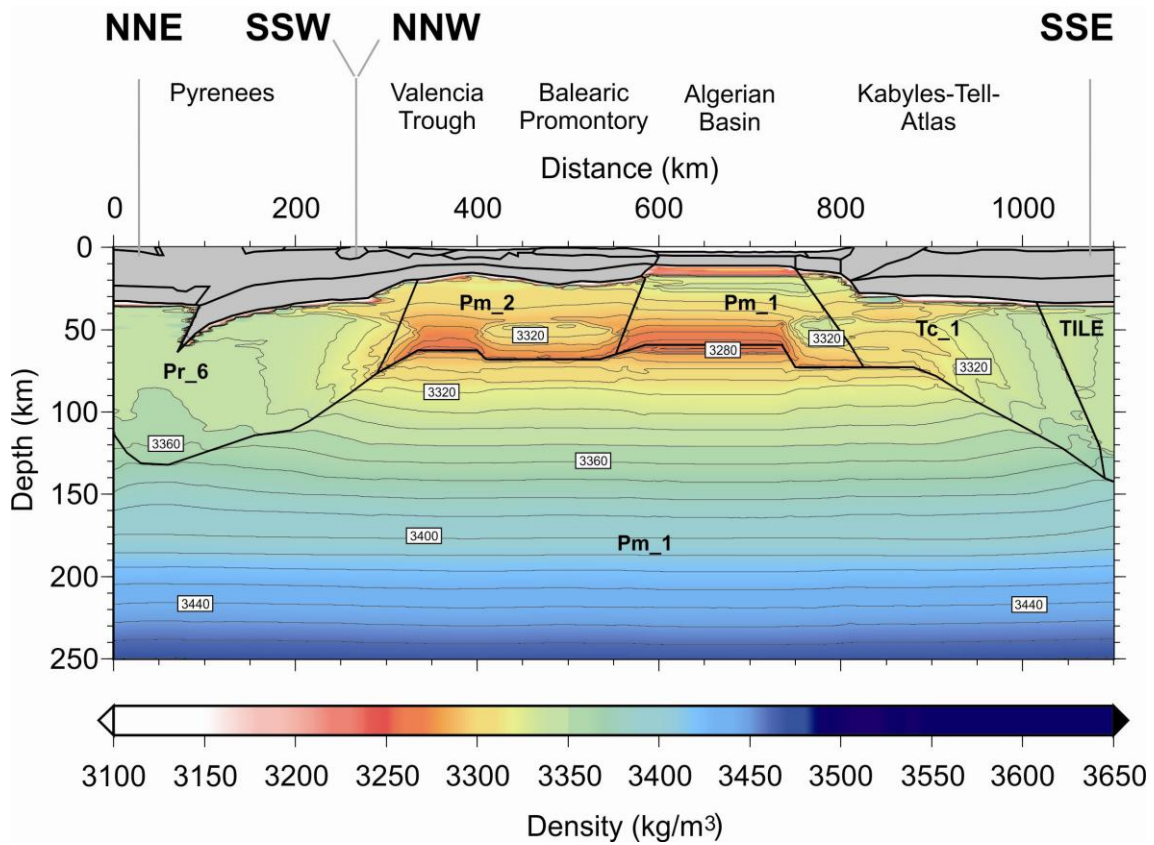
Figure 2.7: Calculated mantle density distribution along the modeled transect. Contour lines every 10 \text{ kg m}^{-3} . Sharp density increase in the uppermost mantle beneath the Algerian Basin is related to the Pg–Sp phase transition. Sharp density increase at \sim 50 \text{ km} depth is related to Sp–Grt phase transition.
