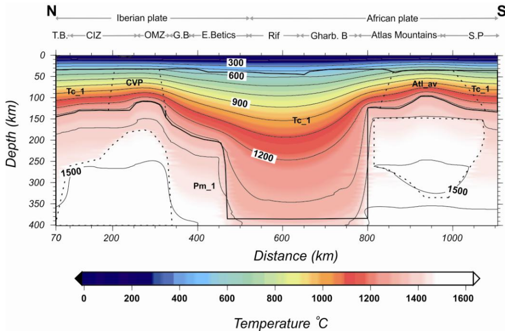
Figure 5.6: Calculated temperature distribution along the Iberian Massif-Arc of Gibraltar-Atlas Mountains geo-transect and mantle domains with different Tc chemical composition (see Table 5.2). Contour lines every 100 °C.
