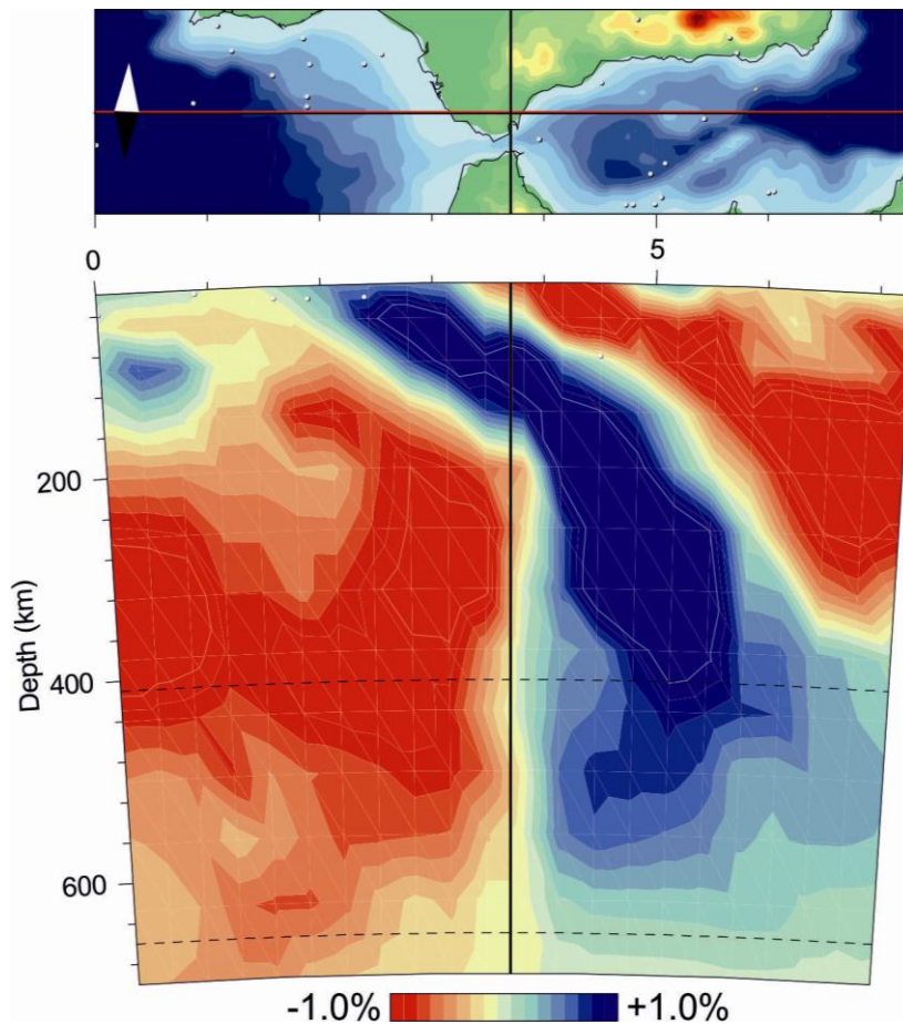
Figure 5.5: East to west tomographic cross-section based on the tomographic model of Villaseñor et al. (2003). Black line shows the location of the Iberian Massif-Arc of Gibraltar-Atlas Mountains geo-transect.
