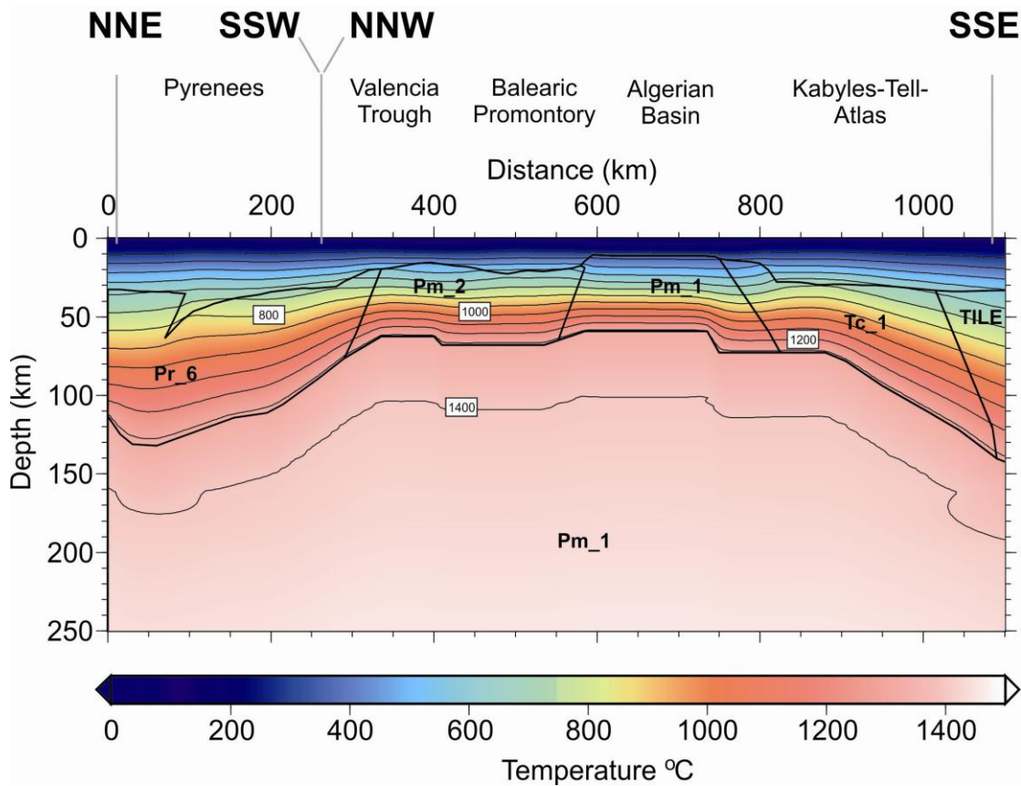
Figure 2.6: Calculated temperature distribution along the modeled transect. Contour lines every 100 °C.
