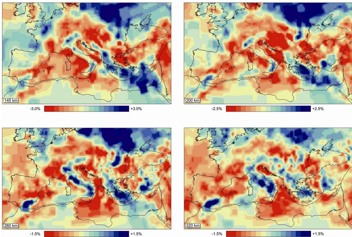
Figure 1.2: P-wave anomaly of the western-Mediterranean region from the tomography model of Villaseñor et al., 2003 for different depths (145, 200, 260 and 320). Shown are P wave seismic velocity anomalies relative to the 1-D reference model ak135 of Kennett et al. (1995). The blue anomaly under the Rif-Gibraltar-Betic (RGB) (southern Iberia) is the image of the slab. Courtesy by A. Villaseñor.
