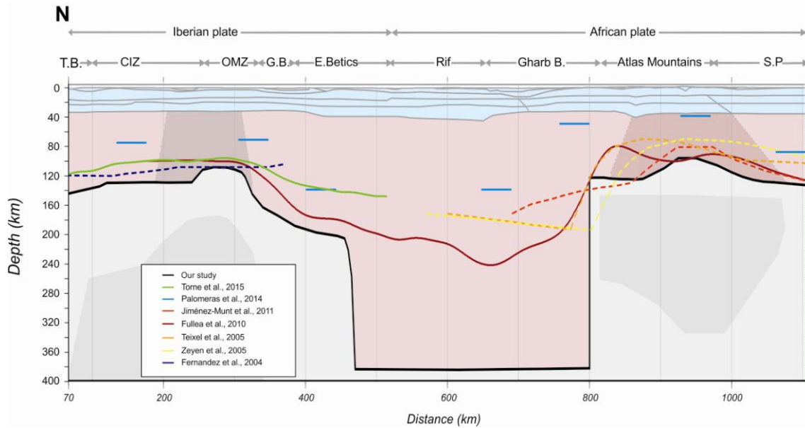
Figure 5.11: Calculated topographies of the lithosphere-asthenosphere boundary from different models. Dashed lines correspond to profiles that do not coincide with the direction of the Iberian Massif-Arc of Gibraltar-Atlas Mountains geo-transect. CIZ, Central Iberian Zone; OMZ, Ossa Morena Zone; GB, Guadalquivir Basin; S.P, Sharan Platform.
