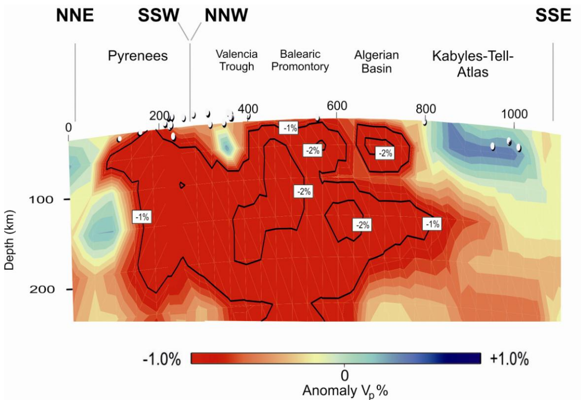
Figure 2.3: P-wave tomography model along the profile (Villaseñor et al., 2003).
