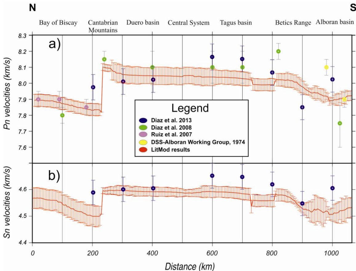
Figure 4.9: a) Pn velocities along the geo-transect. Red line indicates calculated Pn values with the associated standard deviation of the first 15 km of the uppermost mantle. Circles with error bars denote Pn-values from seismic experiments (see legend); b) Sn velocities along the modeled transect. Red line indicates calculated Sn values. Symbols with error bars denote Sn-values from Diaz et al., 2013.
