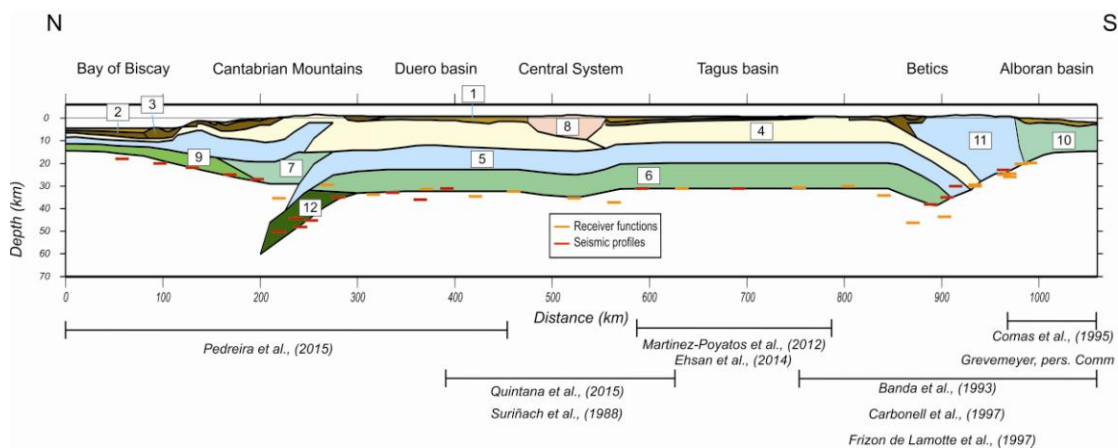
Figure 4.2: Crustal structure corresponding to the best fitting model. Different bodies have been modeled using geological cross-sections (overlaid) and seismic experiments (see text for details). Physical properties of crustal bodies are reported in Table 4.1.
