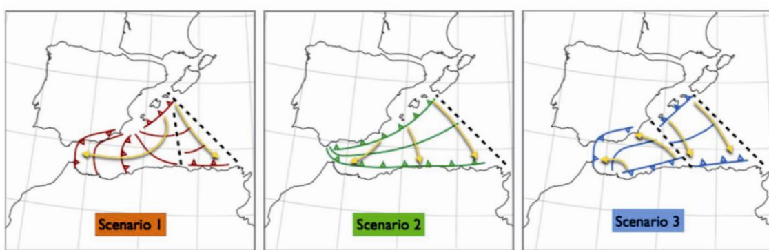
Figure 1.4: An illustration of rollback as portrayed in the three different reconstruction scenarios from Chertova et al., 2014. Scenario 1 (Spakman and Wortel, 2004) and scenario 2 (Faccena et al., 2004) assume a unique subduction polarity but start from different initial subduction zone (short and long respectively). Scenario 3 (Vergés and Fernandez, 2012) shows two opposite dipping subductions. Dashed lines represent proposed transform fault regions. The triangular zone between the transform zones of Scenario 1 depicts the lithosphere that rolls back toward the east Kabyliides (Spakman and Wortel, 2004).
