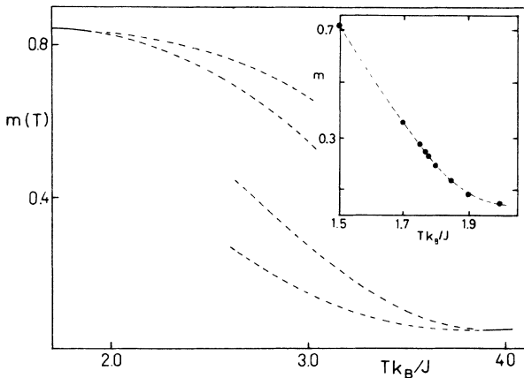
FIG. 7. Discontinuous phase transitions showed up by the model in case 4 (as defined in Sec. III) when x=0.125 . The dashed lines in the main graph represent upper and lower bounds to the data obtained from different independent runs. The inset shows the situation when the concentration of fixed up spins is 0.049 53 and the one for fixed down spins is 0.050 47.
