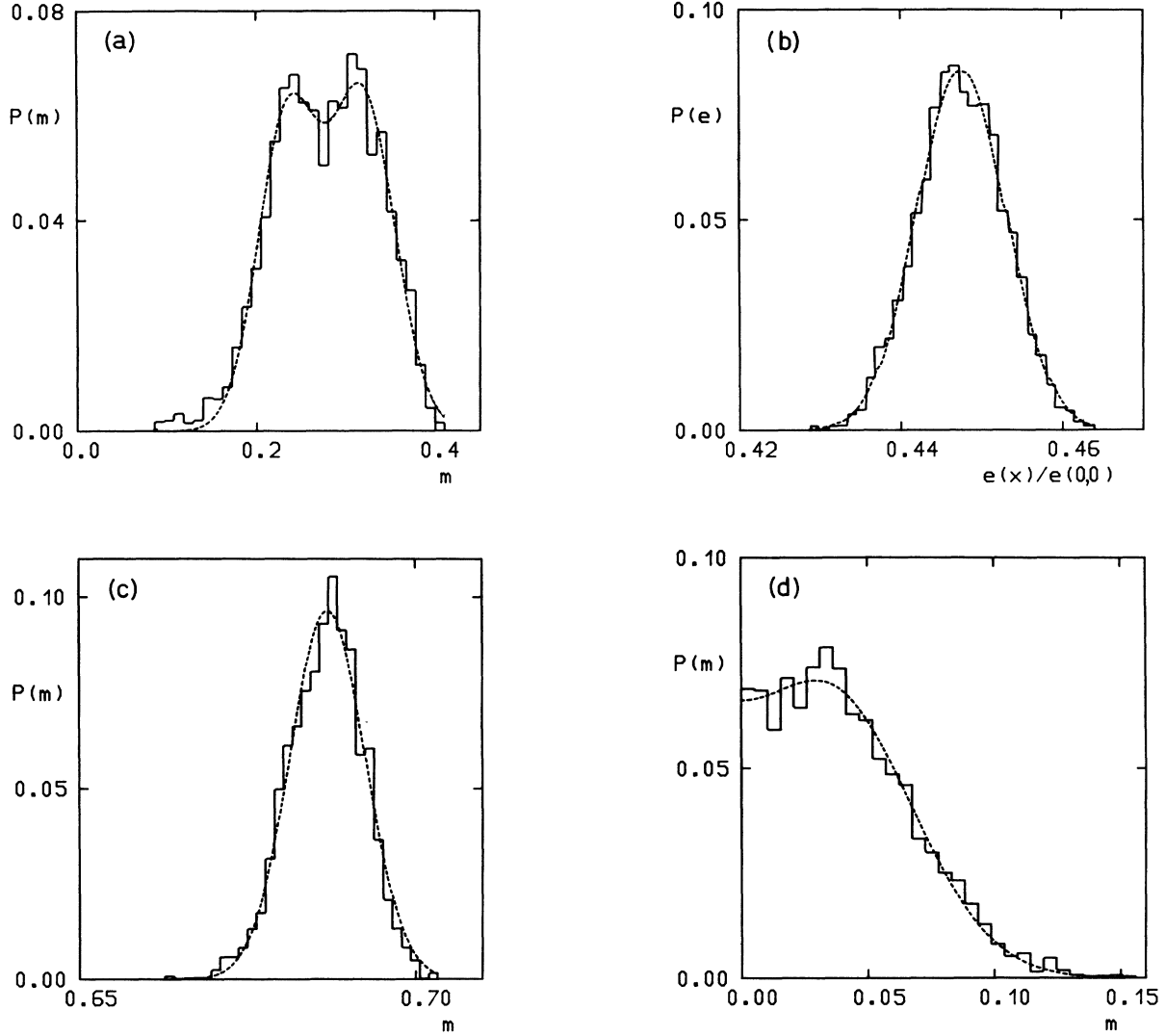
FIG. 12. Distribution of measured values and fitted Gaussians for the “blocked” system with l=4 : (a) magnetization values for T=0.997 T_c , (b) energy values for the same temperature, (c) magnetization values for T=0.882 T_c , and (d) magnetization values for T=1.058 T_c .
