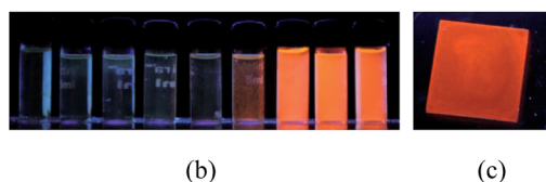
Fig. 5 (a) PL spectra of 2 in MeOH/water mixed solvents with different f_w (water fraction). Inset: variation of PL intensity with respect to different water fraction. (b) Luminescent images of 2 in different water fraction (c) image for a solid sample of 2 under irradiation with a 365 nm UV lamp; [ c = 10 \times 10^{-5} M].
