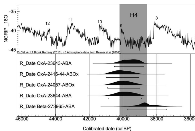
Fig. 2. Plot of the Canyars ^{14}\text{C} dates, calibrated with the Intcal09 curve (Reimer et al., 2009) and compared with the North Greenland Ice Core Project (NGRIP) \delta^{18}\text{O} ice-core record of Svensson et al. (2006) and Andersen et al. (2005), showing GI interstadials and Heinrich Event 4 according to Svensson et al. (2008) (prepared using OxCal vs. 4.1.7; Bronk Ramsey, 2009).
